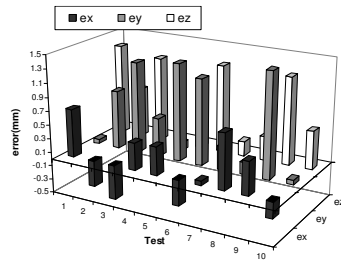
Fig.5: The error schematics in x, y, z directions for forward kinematics tests.
