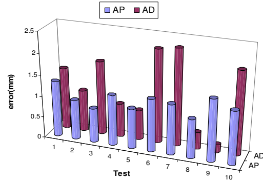
Fig.10: Position and distance accuracy investigated in positioning tests according to ISO9283.
