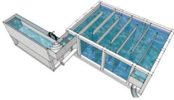
Fig 1. Geometric Contact Tank Model CT-1 [1].
