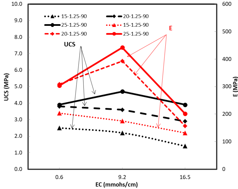
Fig. 1. Effect of water salinity on the UCS and modulus of elasticity (E) of soilcrete
