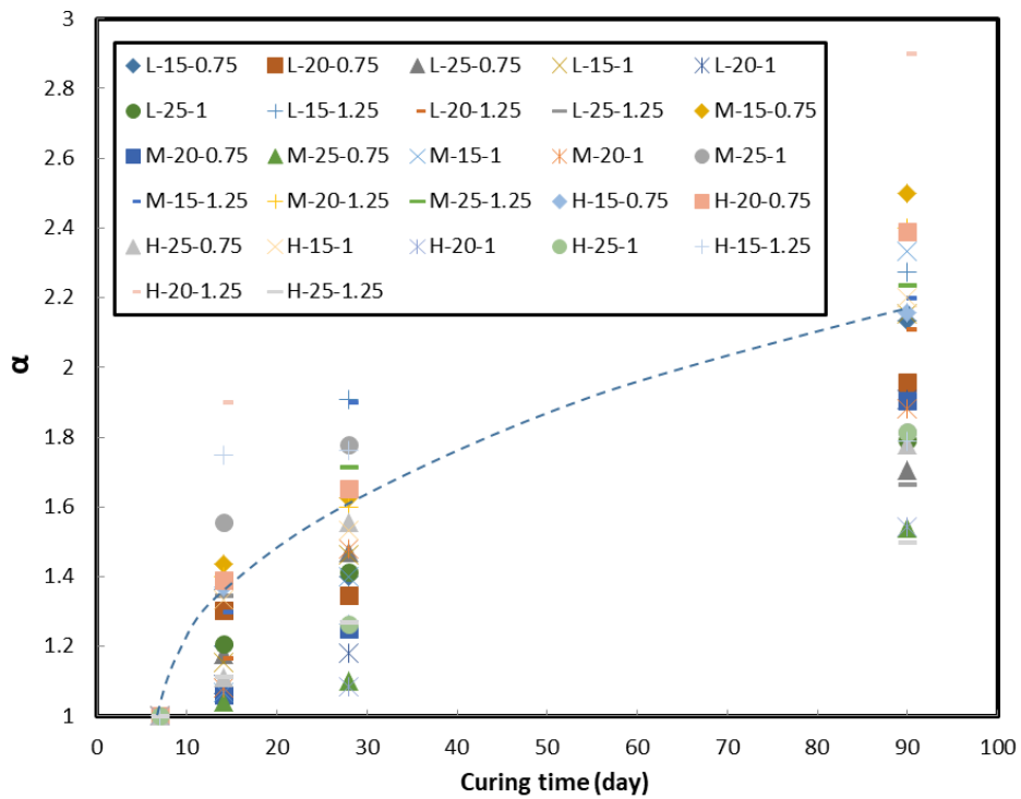
Fig. 2. Effect of water salinity on the strength of soilcrete vs. curing time
