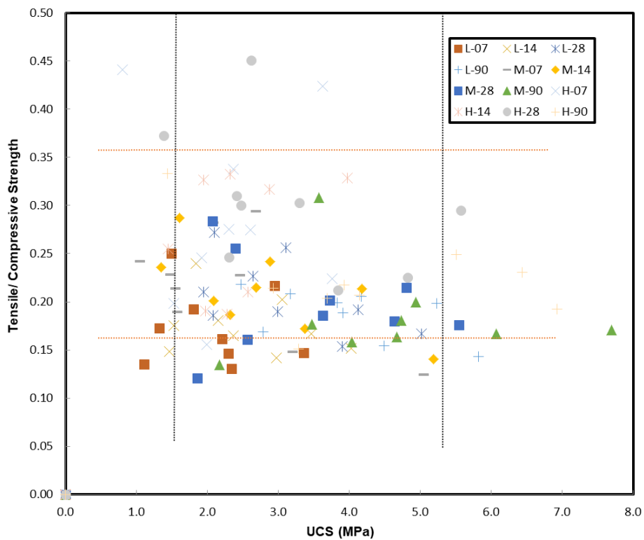
Fig. 3. Relation between UCS and tensile strength in soilcrete
