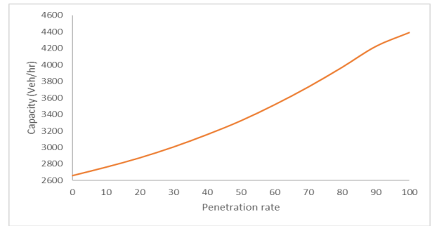
Fig. 2. Impact of AVs on the capacity of merge section
