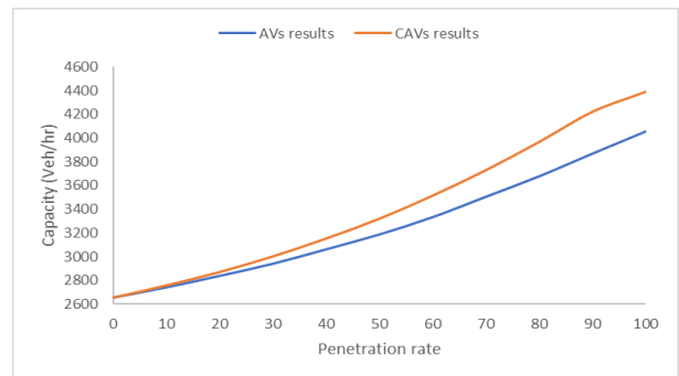
Fig. 3. Impact of AVs on the capacity of merge section
