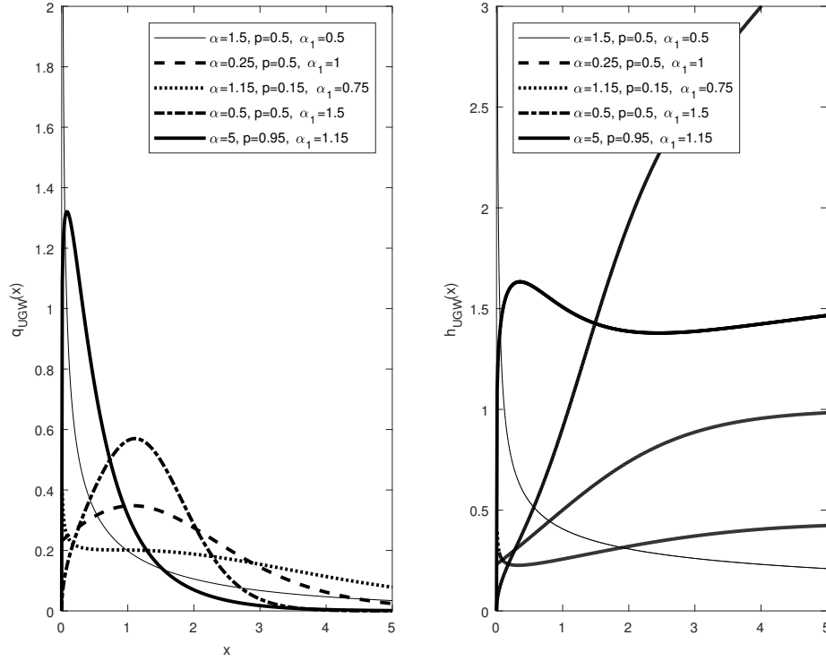
Figure 4: Density (left) and hazard rate function (right) of UGW(\alpha, p, \alpha_1, \beta_1) distributions for \beta_1 = 1 and some other parameters values.
