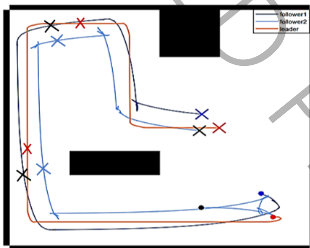
Fig. 9. Simulation of mobile robots' trajectory in a virtual environment without disturbance for followers with PID controller
