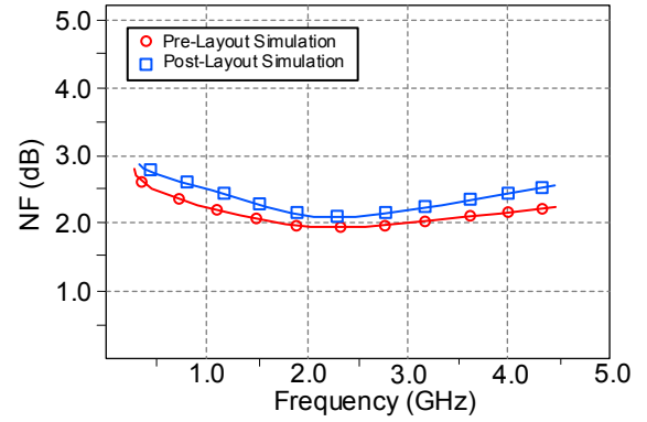
Fig. 11. Simulated noise figure in two schematic and post-layout simulation modes
