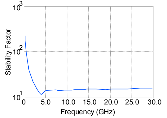
Fig. 14. Post-layout simulation of Rollett stability factor (Kf) of the proposed circuit
