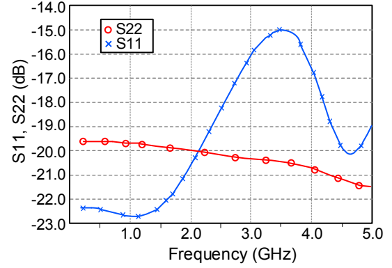
Fig. 10. Simulation results for input and output return losses
