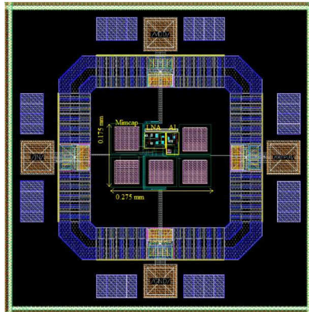
Fig. 16. The layout of the proposed LNA
