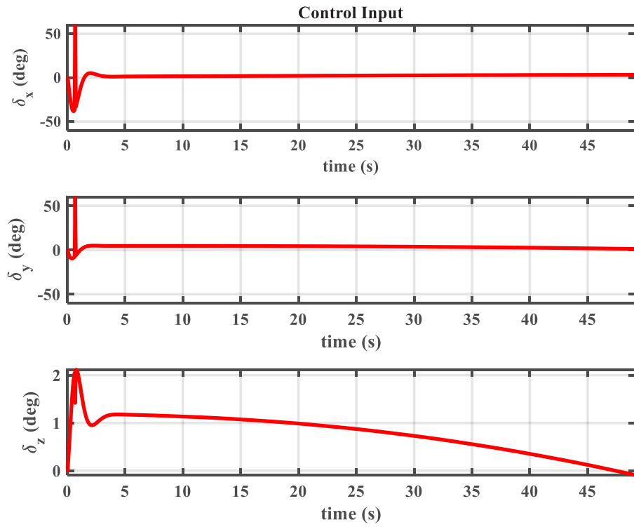
Fig. 5. Missile control input - PID controller
