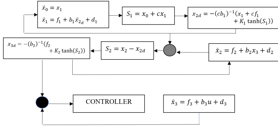
Fig. 2. Controller block diagram[14][14](Ma, et al. 2020)
