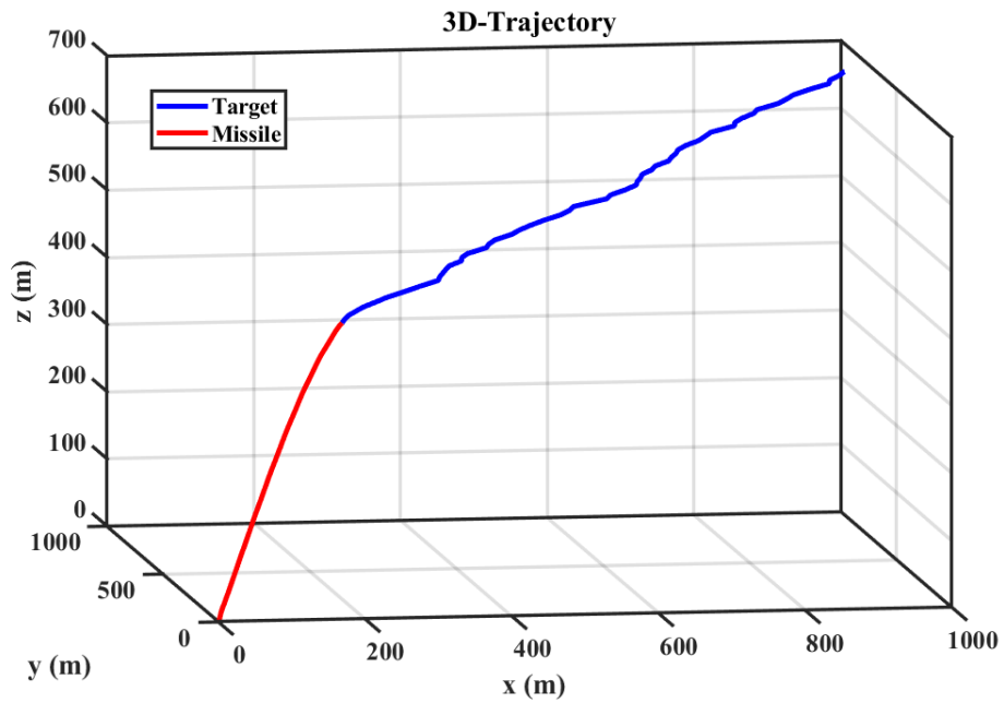
Fig. 6. Missile trajectory and target - PID controller
