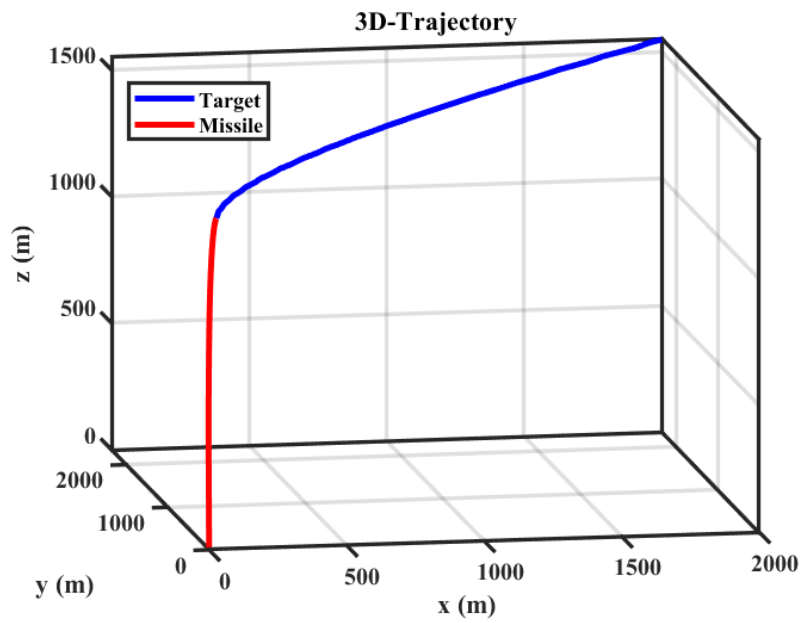
Fig. 11. Missile-target trajectories using the LQR controller
