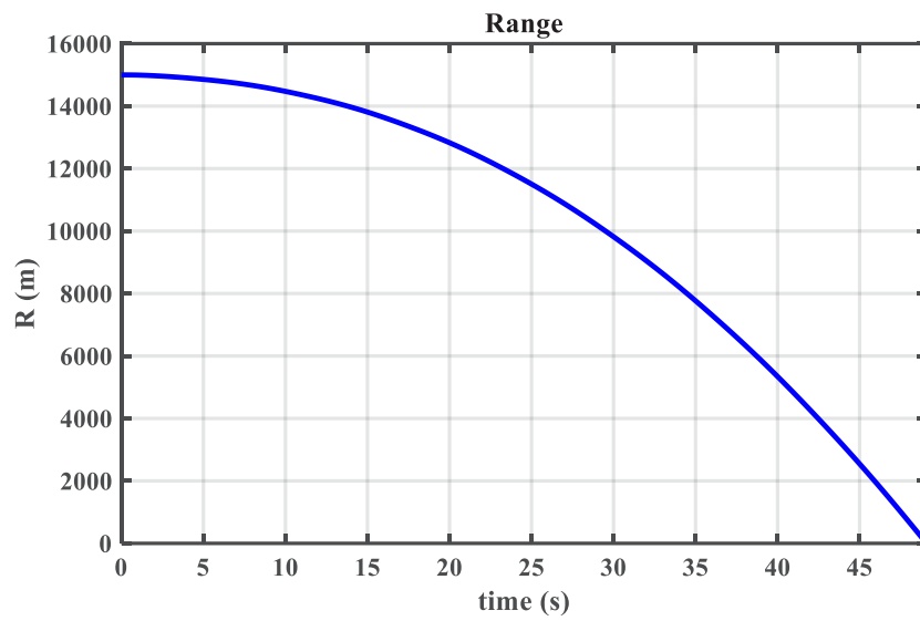
Fig. 3. The relative distance of the missile and the target - PID controller
