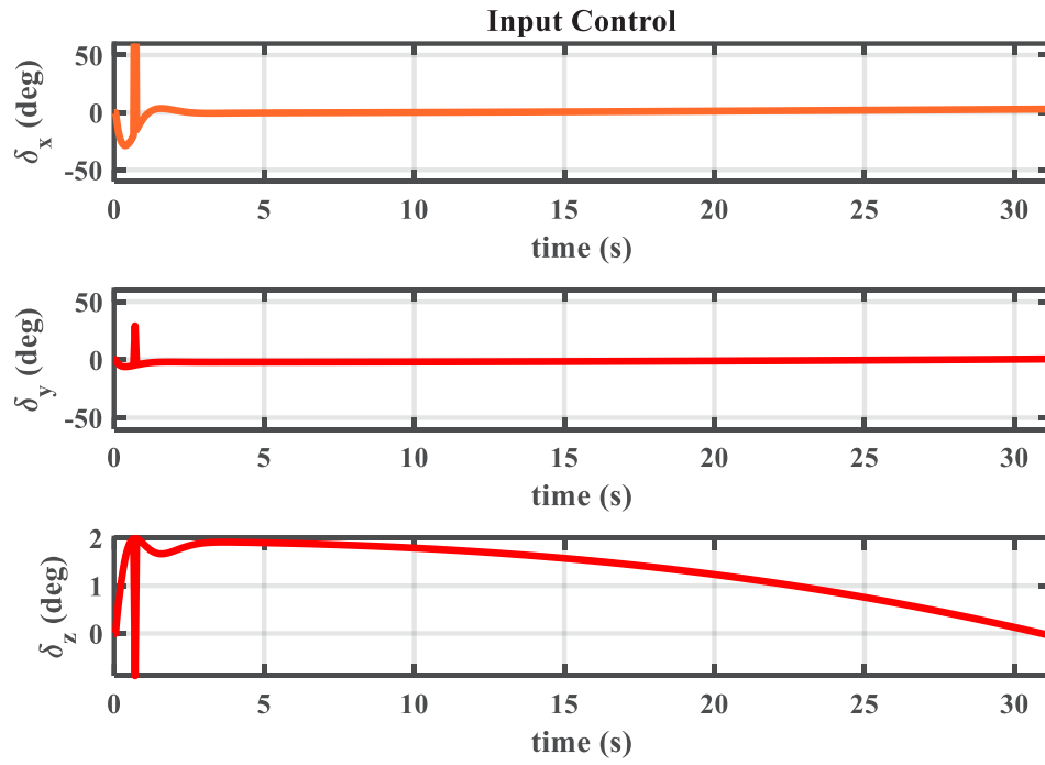
Fig. 10. Missile control input with the LQR controller
