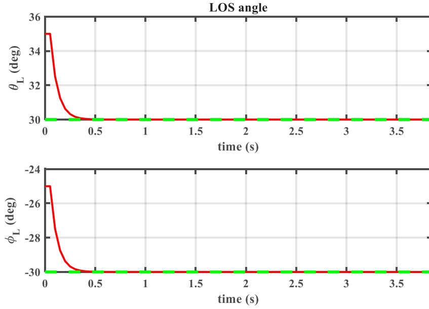
Fig. 13. Changes of elevation and side angles with time using the implicit predictive model controller
