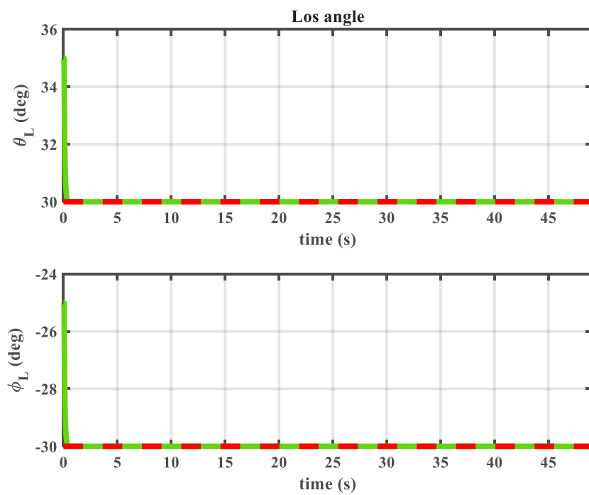
Fig. 4. Changes of elevation and side angles - PID controller
