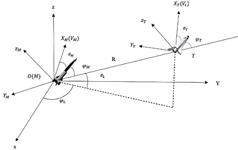
Fig. 1. Kinematics of conflict
