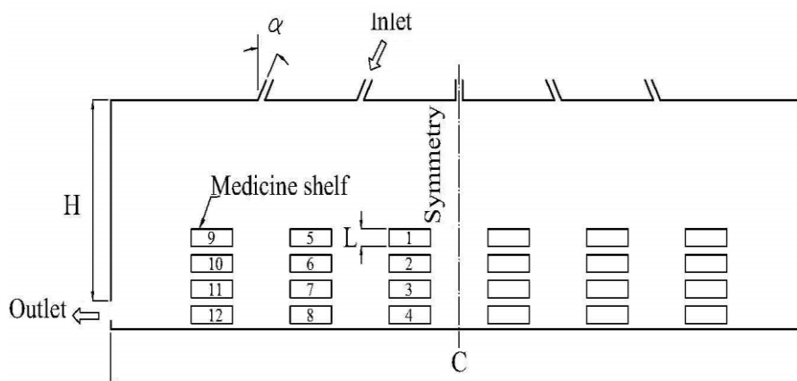
Fig. 1. Pharmaceutical warehouse and shelves, and grilles arrangement
