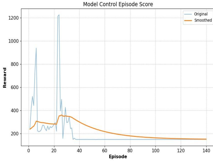
Fig. 4. The acquired reward during model control episodes, in the presence of DQN algorithm
