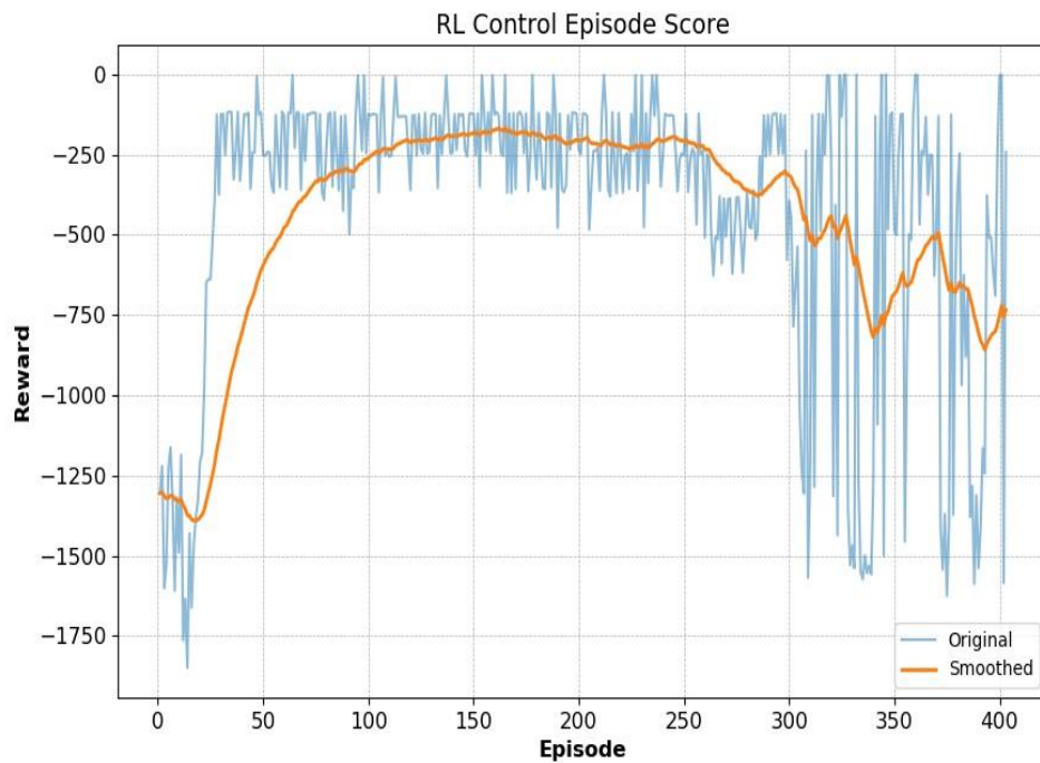
Fig. 5. The obtained reward during RL control episodes using the DDPG algorithm with untuned hyperparameters
