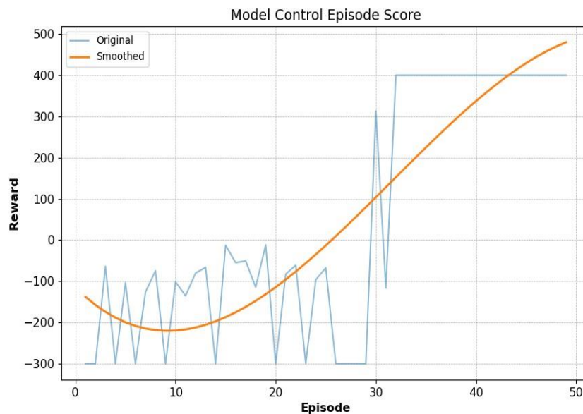
Fig. 14. The acquired reward during model control episodes, in the presence of TD3 algorithm
