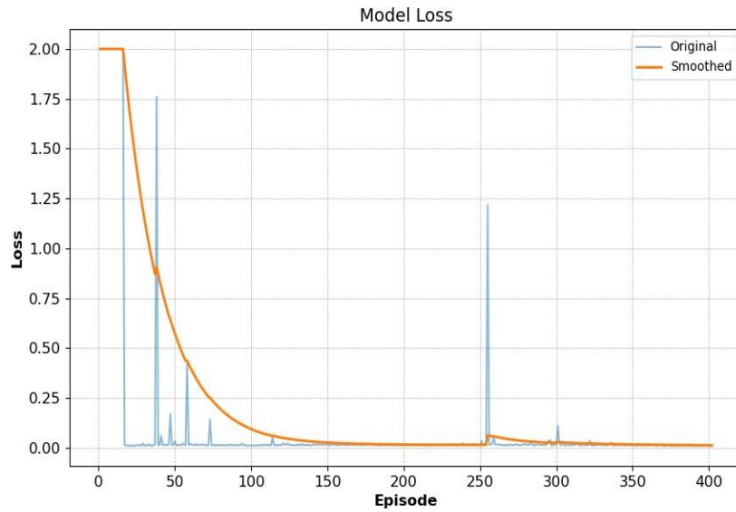
Fig. 13. The environment model loss using the suggested framework, in the presence of TD3 algorithm with tuned hyperparameters
