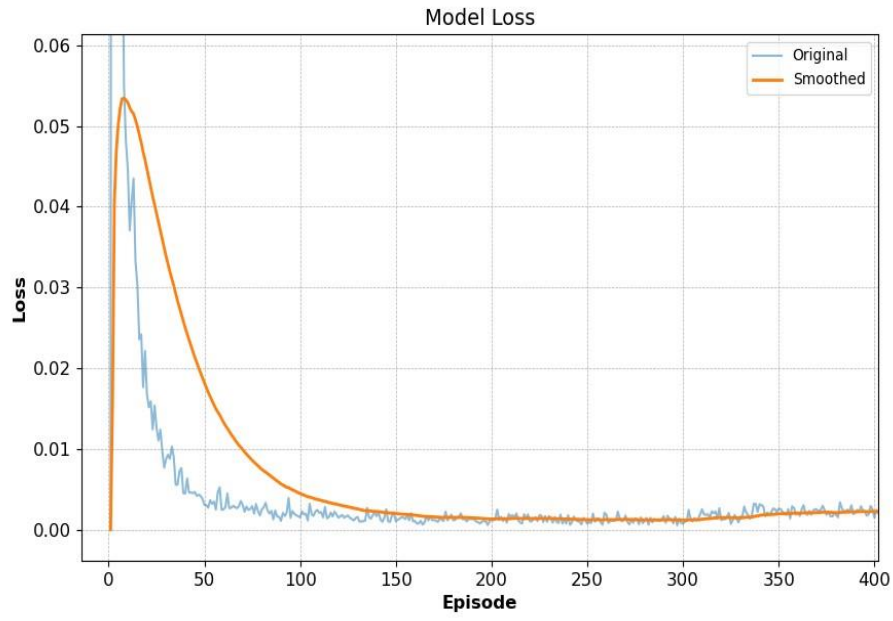
Fig. 7. The environment model loss using the suggested framework, in the presence of DDPG algorithm with untuned hyperparameters
