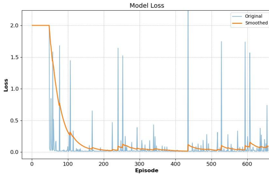
Fig. 12. The environment model loss using the suggested framework, in the presence of TD3 algorithm with untuned hyperparameters
