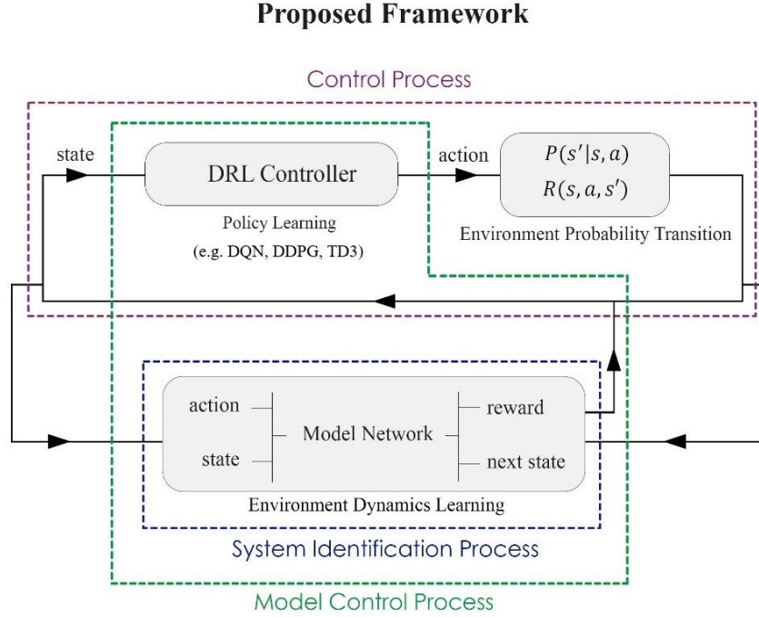
Fig. 1. Block diagram of the proposed framework (Remark: the policy learning in DQN algorithm is done via Q-network, while the policy is learned via actor and critic networks in DDPG and TD3 algorithms)
