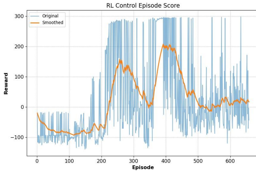
Fig. 10. The obtained reward during RL control episodes, in the presence of TD3 algorithm with untuned hyperparameters
