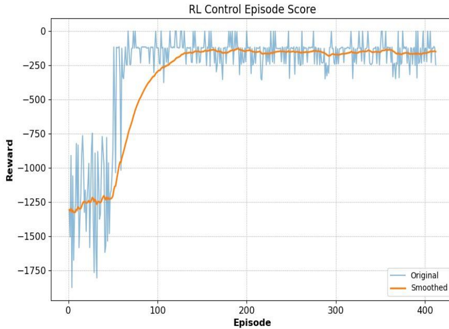
Fig. 6. The obtained reward during RL control episodes using the DDPG algorithm with tuned hyperparameters
