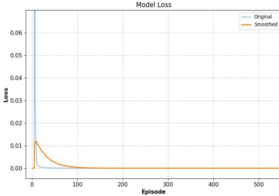
Fig. 3. The environment model loss using the suggested framework, in the presence of DQN algorithm
