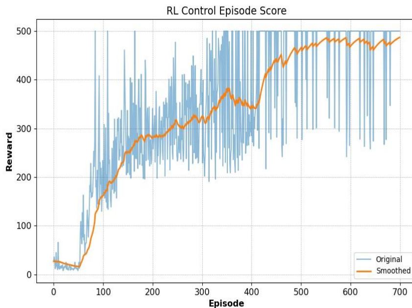
Fig. 2. The obtained reward during RL control episodes, in the presence of DQN algorithm
