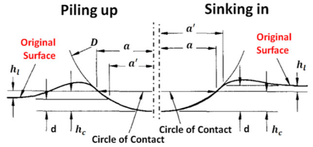
Fig. 2. Schematic of the geometry of the depression around the penetrator.
