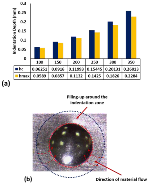
Fig. 4. a) Comparison of calculated instantaneous penetration values based on analysis with the value measured during the penetration test, b) Image of deformation created around the penetration area.
