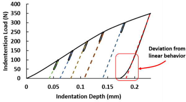
Fig. 1. Measured load-penetration depth diagram and linear fit of the initial part of the load-discharge diagram.
