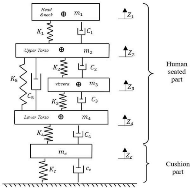
Fig. 8. 5 DOF human and cushion model
