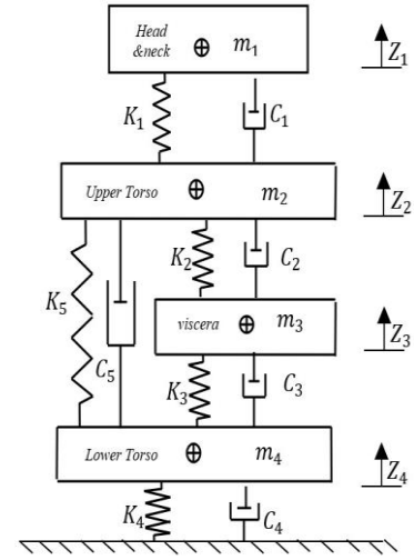
Fig. 1. 4 DOF wan-schimmels model [10].
