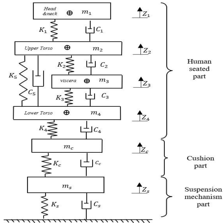
Fig. 10. 6 DOF human and seat suspension and cushion model.
