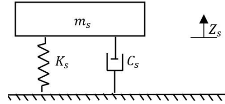
Fig. 3. Seat suspension mass-spring model
