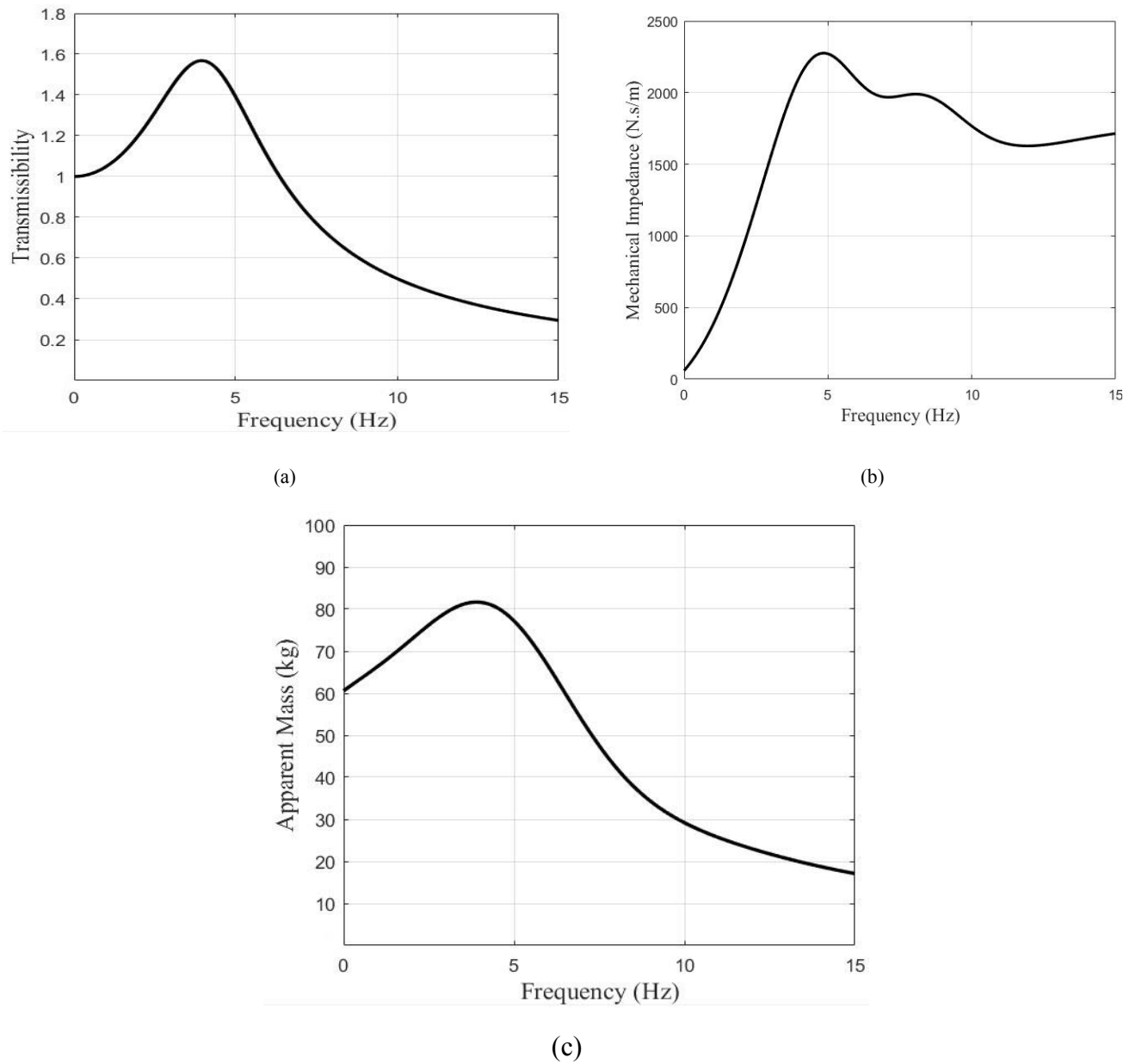
Fig. 5. (a) seat-to-head transmissibility of a human seated without considering the effect of the seat suspension and cushion. (b) Mechanical impedance of a human seated without considering the effect of the seat suspension and cushion. (c) Apparent Mass of a human seated without considering the effect of the seat suspension and cushion.
