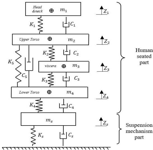
Fig. 6. The 5 DOF human and seat model
