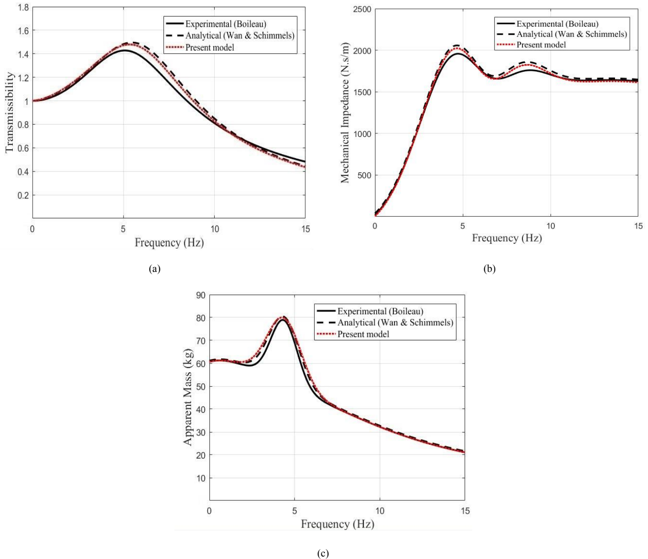
Fig. 4. (a) Validation of the analytical model of seat-to-head transmissibility by comparison with experimental and analytical models. (b) Validation of the mechanical impedance. (c) Validation of the apparent mass.
