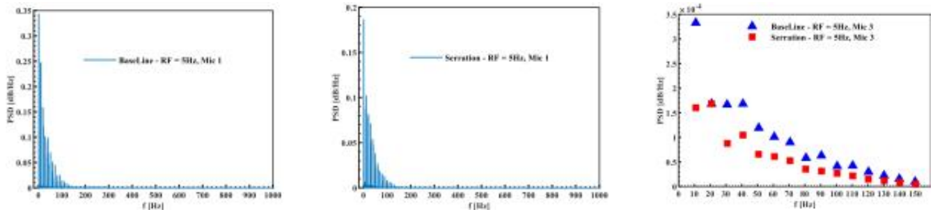
Fig. 6. PSD plots versus flow frequency, Left) baseline model, middle) serration model, right) energy peaks between the baseline and serration models.
