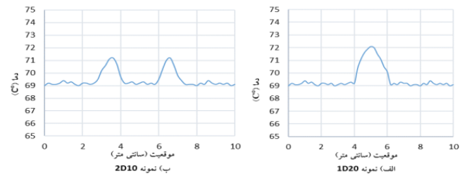
Fig. 3. Numerical results of surface temperature changes along the line passing through the center of the defects of the samples.
