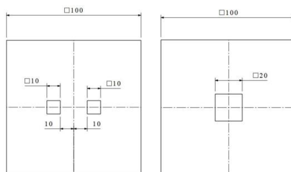
Fig. 1. Schematic image of the location of defects.
