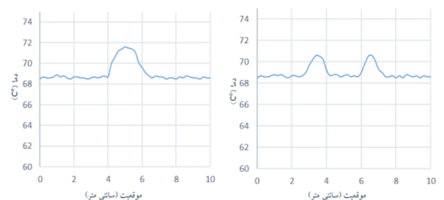
Fig. 4. Thermographic test results and temperature change curve on the line passing through the center of the defects on the surface of the samples.
