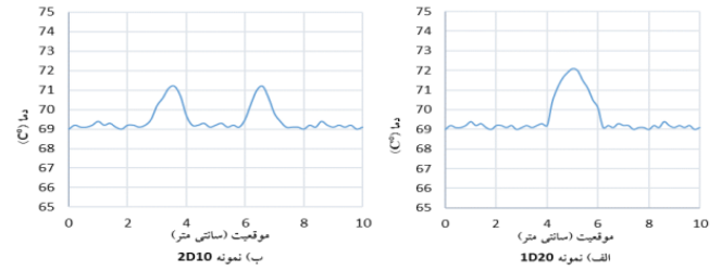
Fig. 3. Numerical results of surface temperature changes along the line passing through the center of the defects of the samples.
