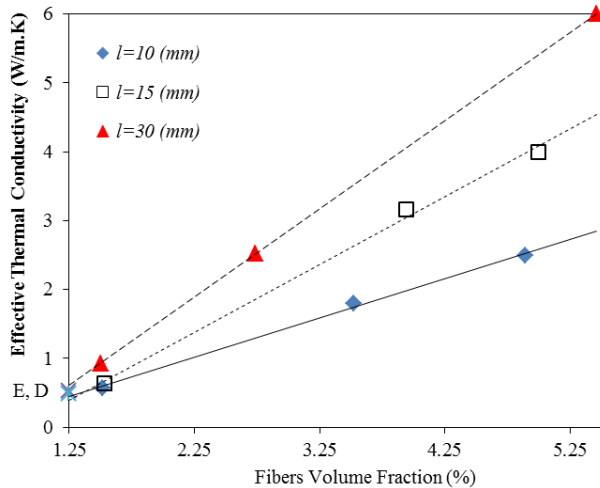
Fig. 4. The effect of length and volume fraction of copper fibers on the effective thermal conductivity of a fibrous composite ( d = 0.15 mm).
