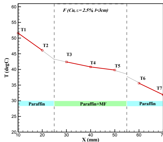
Fig. 3. Steady-state temperature distribution for a Paraffin/Copper fibrous composite.
