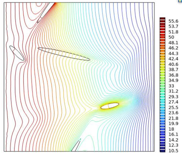
Fig. 5. Steady-state temperature distribution of a fibrous composite in the solid state.
