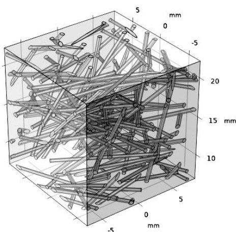
Fig. 2. 3D numerical model of the fibrous composite.
