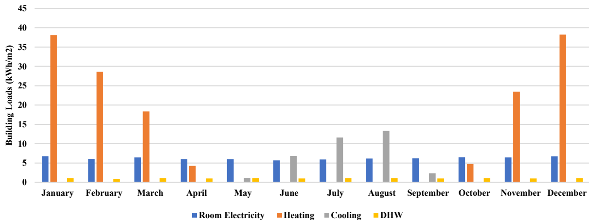
Fig. 8. summarizes the monthly normalized energy consumption of the building with PCM.
