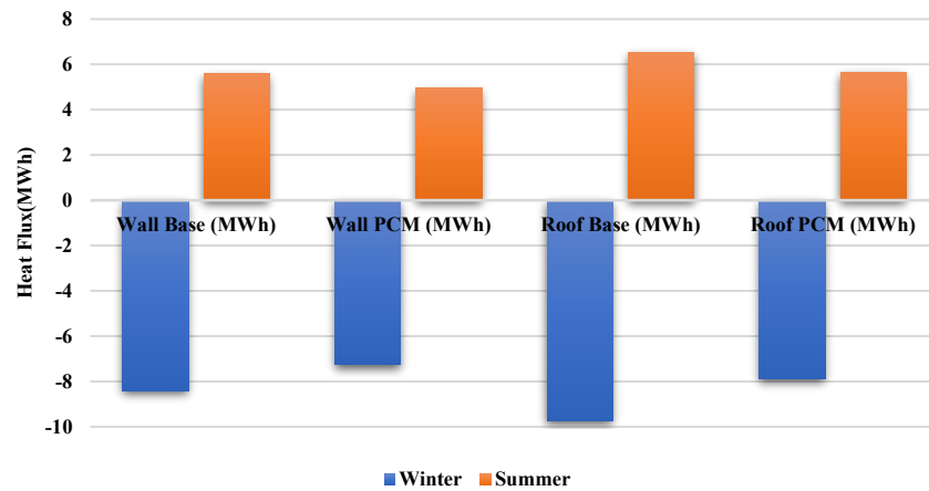
Fig. 6. Seasonal cumulative heat fluxes and percentage reductions due to PCM integration.
