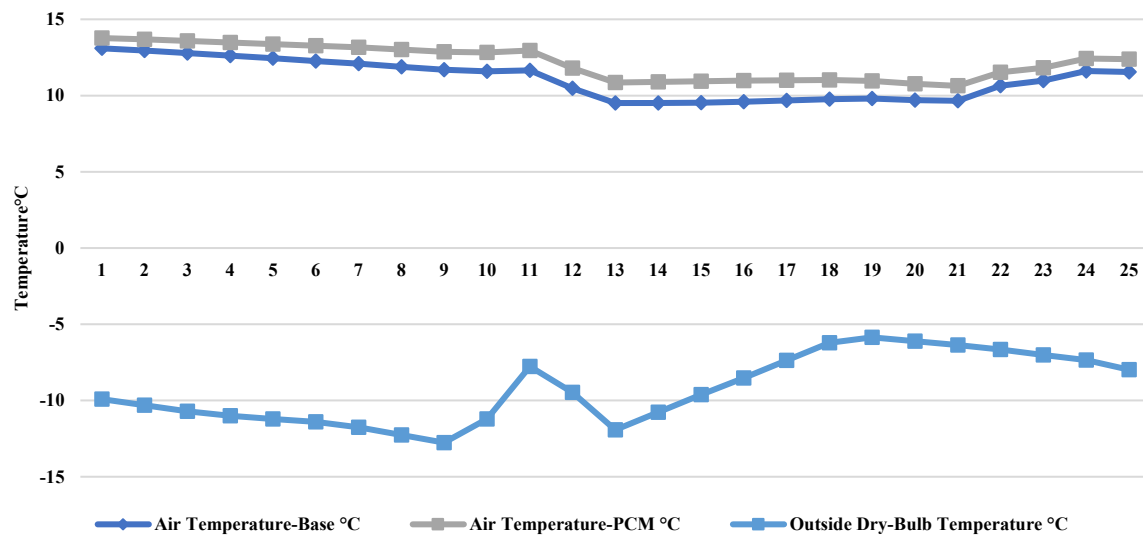
Fig. 10. Hourly temperature profiles for outdoor, indoor baseline, and PCM-integrated indoor environments on December 31st.
