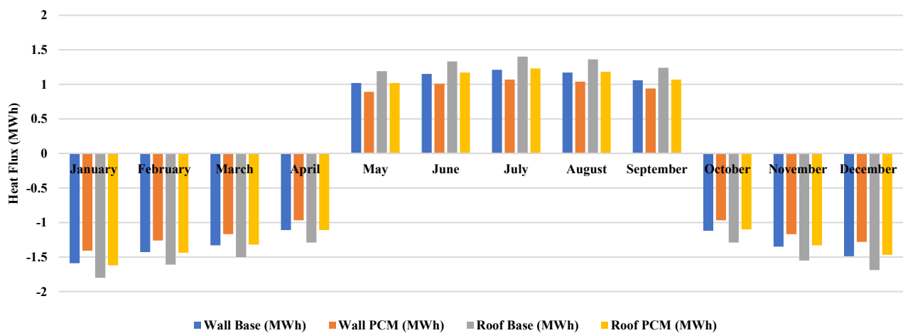
Fig. 5. Monthly heat flux values for walls and roof (Base vs. PCM).
