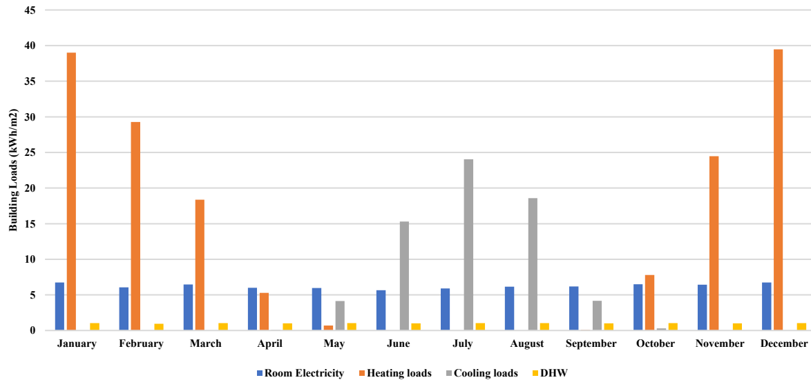
Fig. 7. Summarizes the monthly normalized energy consumption of the building.
