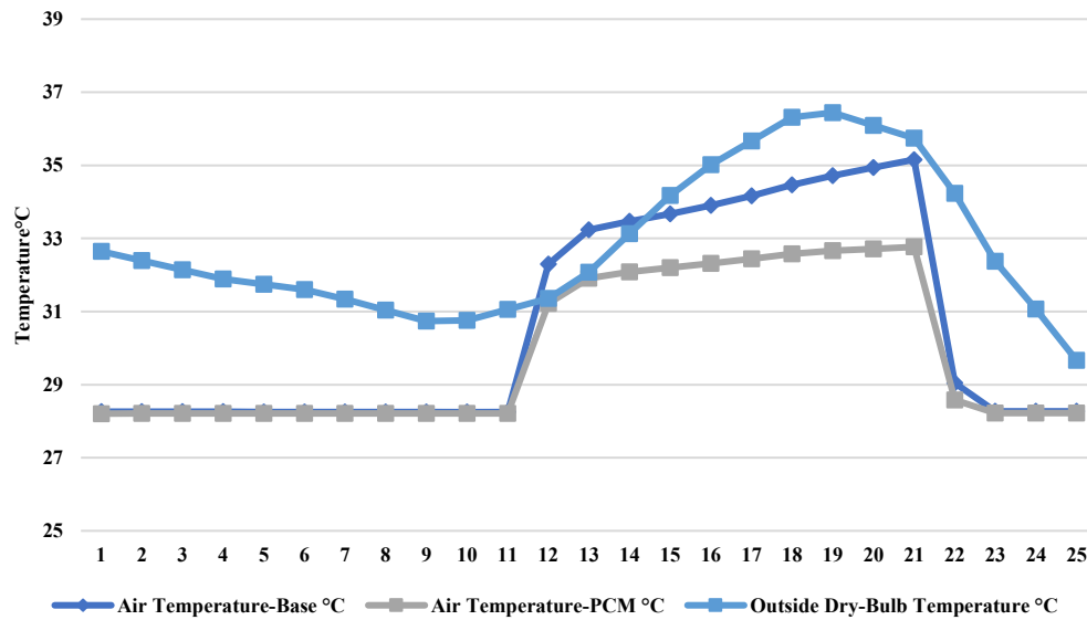
Fig. 9. Hourly temperature profiles for outdoor, indoor baseline, and PCM-integrated indoor environments on July 31 st .
