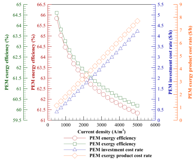
Fig. 4. Effect of variations in current density on the PEM cycle key parameters
