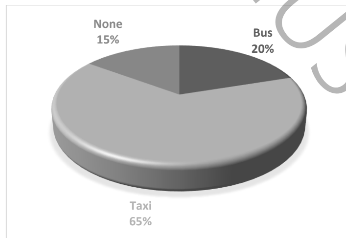
Figure 3: Daily Trips
