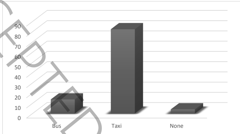
Figure 4: Accessibility
