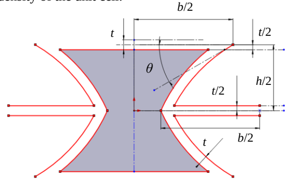
Figure 1. Schematic of a unit cell of two-dimensional curved re-entrant auxetic core (marked with red color).
