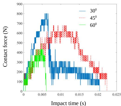
Figure 4. Contact force diagram of sandwich beams with two-dimensional curved re-entrant auxetic after the drop-weight impact test.
