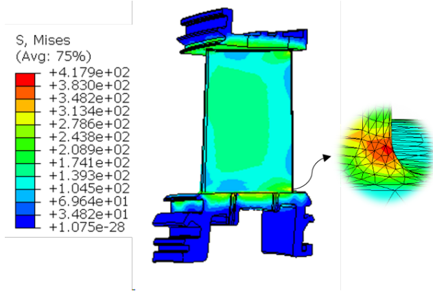
Fig. 1. Von Mises stress distribution at OP 60%.
