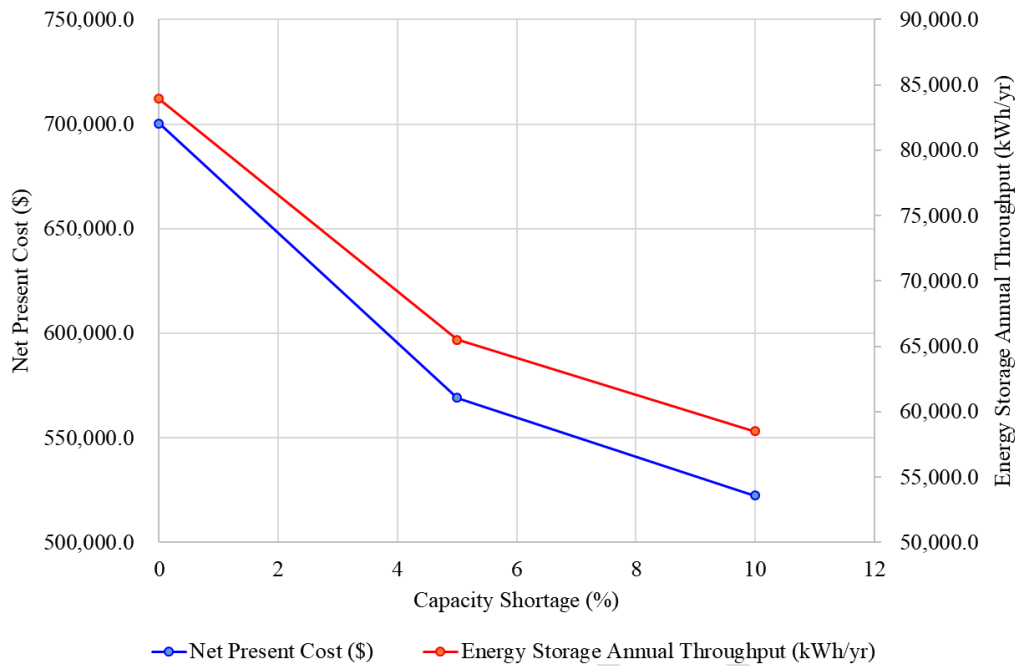
Fig. 9. the variations of NPC and energy storage annual throughput based on maximum annual capacity shortage in scenario #2
