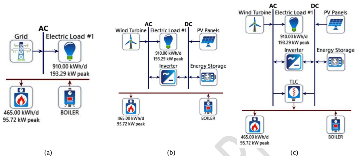
Fig. 2. The schematic of electrical-thermal system architecture (a) Scenario #1 (b) Scenario #2 (c) Scenario #3
