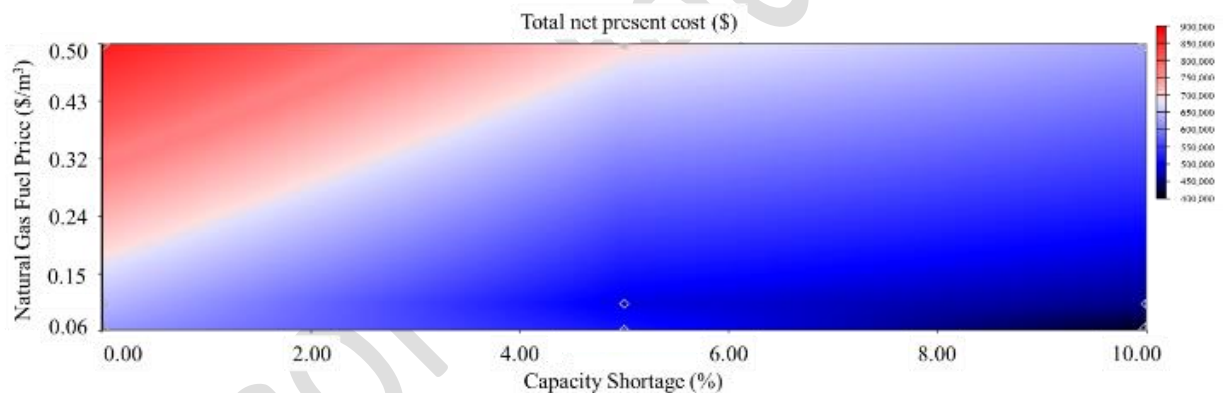
Fig. 11. Surface plot of NPC considering the system reliability and natural gas fuel price variations in scenario #3
