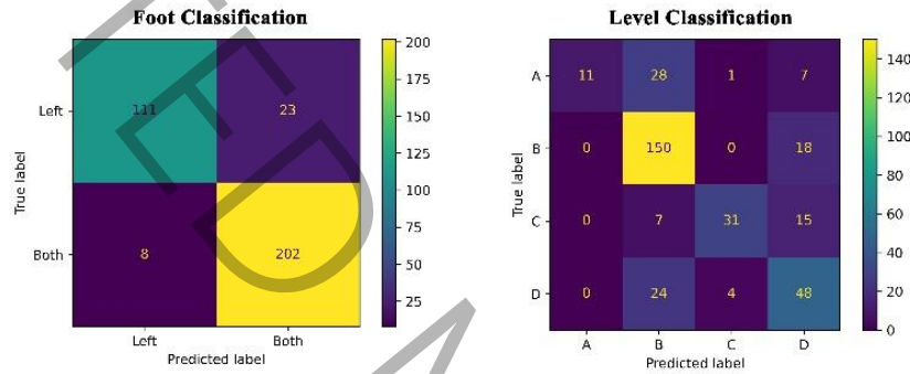
Fig. 6. SVM confusion matrix
