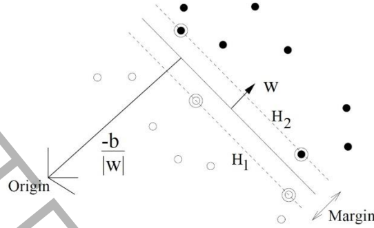
Fig. 5. Linear separating hyperplanes for the separable case. The support vectors are circled [20]
