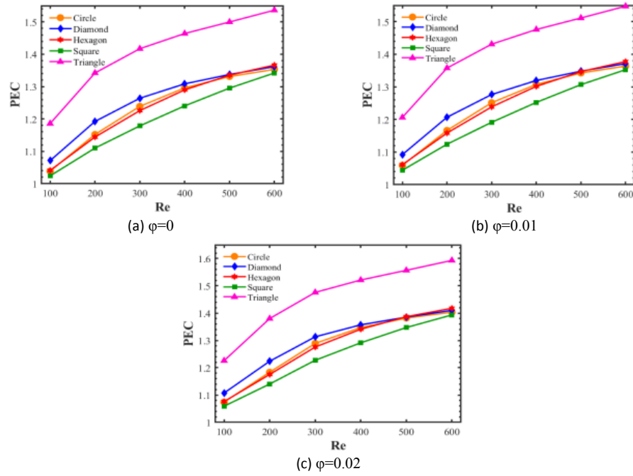
Fig. 4. Effect of interrupted fin shapes on the microchannel performance evaluation criterion at three different volume fractions.
