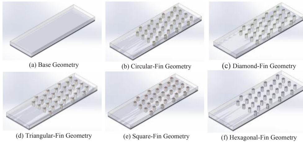
Fig. 1. Isometric view of the different geometries.
