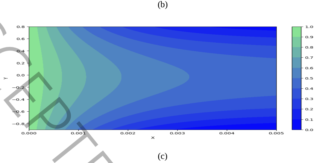
Fig. 14. The effect of changing porosity on the hydrogen concentration contour for Al_2O_3 with porosity percentages of a) 85%, b) 90%, and c) 95%.
