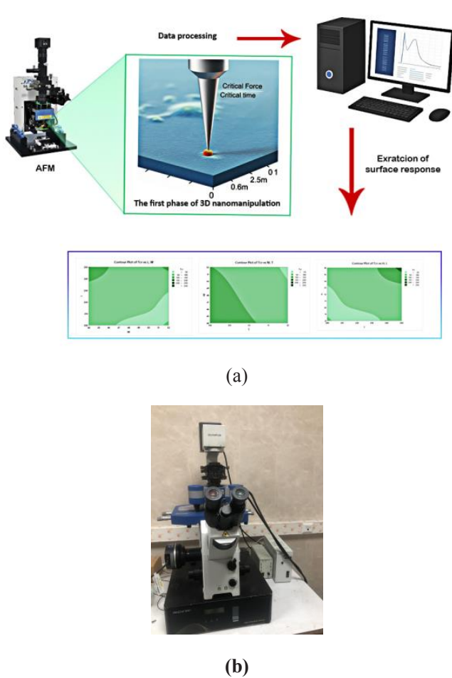
Fig. 1. Schematic representation of the nanoparticle manipulation process and the Atomic Force Microscope (AFM).
