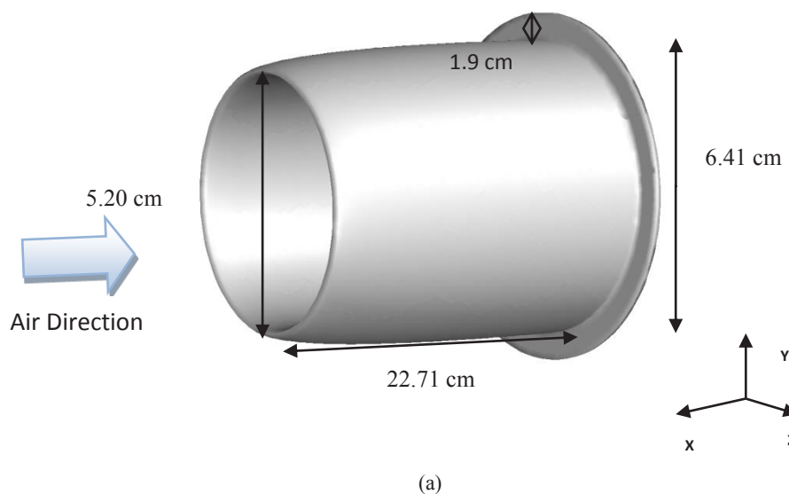
Fig. 1. (a) Angled visualization of the shroud with the flange connected at its terminal, (b) Improved Curved-Flange Configuration. (Continued)
