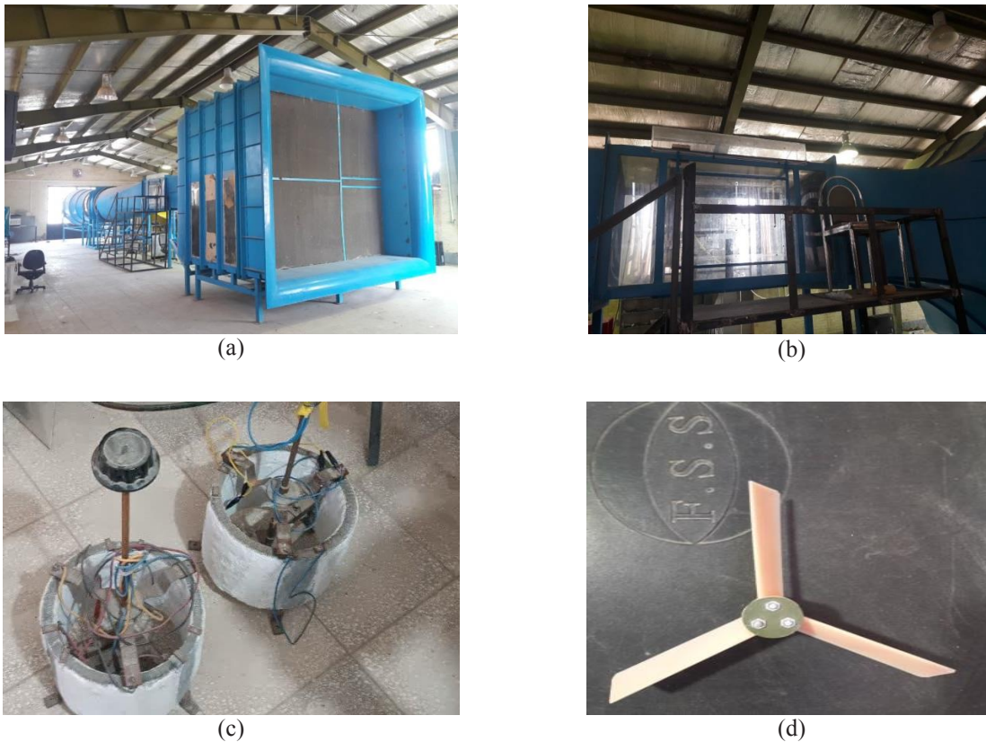
Fig. 2. (a) wind tunnel of Hakim Sabzevari University, (b) wind tunnel test section, (c) rheostat, (d) turbine, (e) digital manometer, (f) pitot tube, (g) mini generator, digital multimeter. (Continued)
