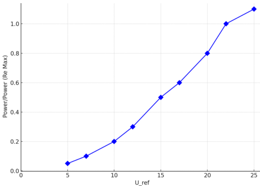
Fig. 5. Turbine power changes with free stream velocity.
