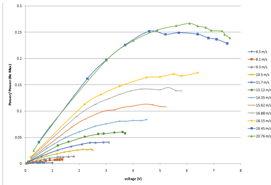
Fig. 6. Variation of turbine power with generator voltage at different wind velocities.
