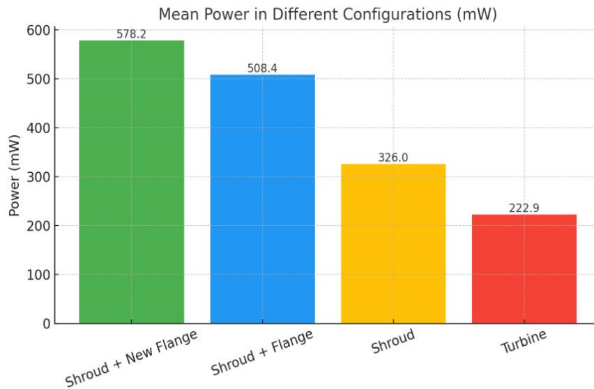
Fig. 11. Average extracted power of the different configurations, expressed in milliwatts.
