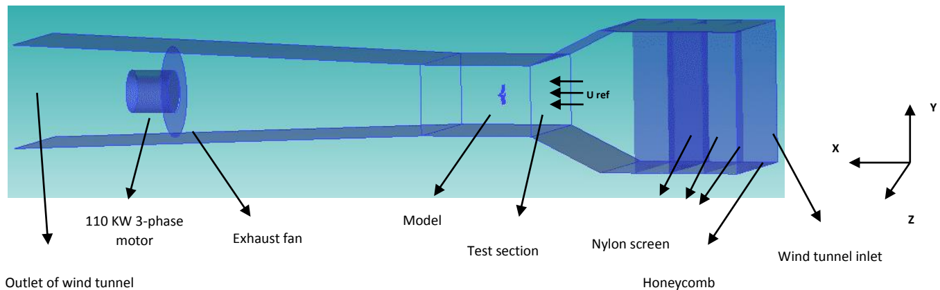
Fig. 3. Schematic of the wind tunnel and its components and the location of the model in the test chamber.
