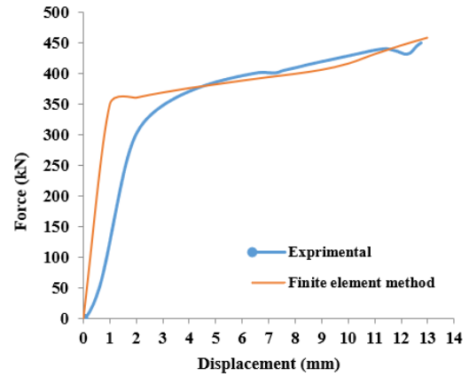
Fig. 2. Comparison of force-displacement diagrams of the absorber.
