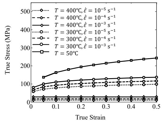
Fig. 1. The effect of temperature and strain rate on stress-strain response of AA3104
