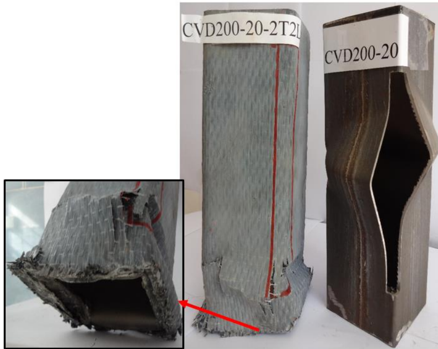
Fig. 11. Failure modes of the specimens with corner deficiency: non-strengthened and strengthened
