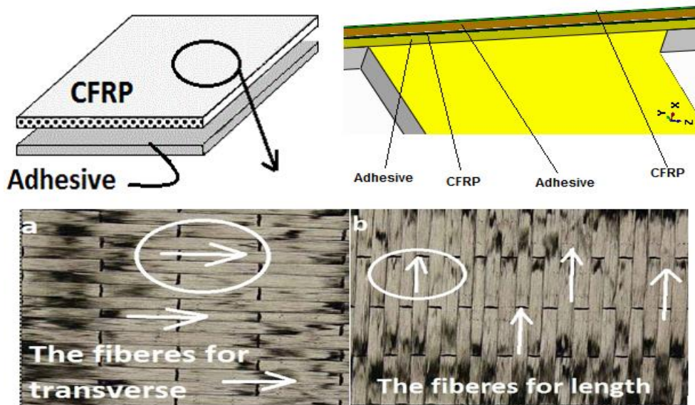
Fig. 2. CFRP sheets: transverse and longitudinal fibers.
