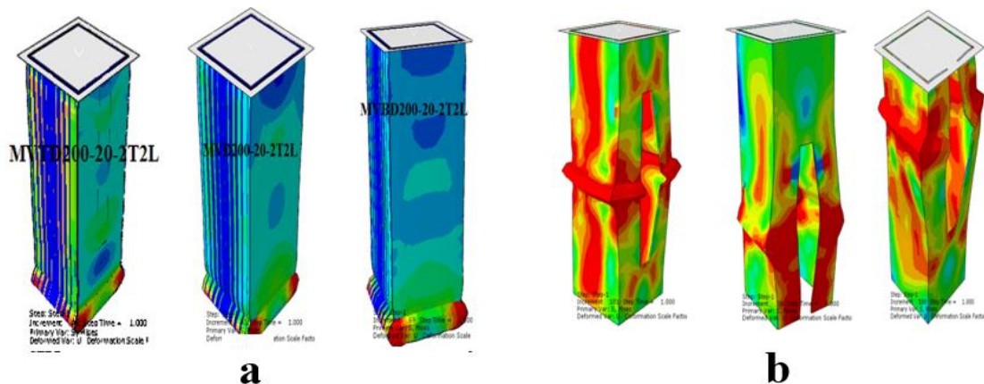
Fig. 12. Deformation of Vertical Deficiency at the Middle Element of Steel Columns (Simulation): (a) strengthened, (b) non-strengthened.
