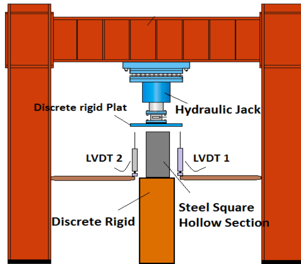
Fig. 3. Experimental test setup.
