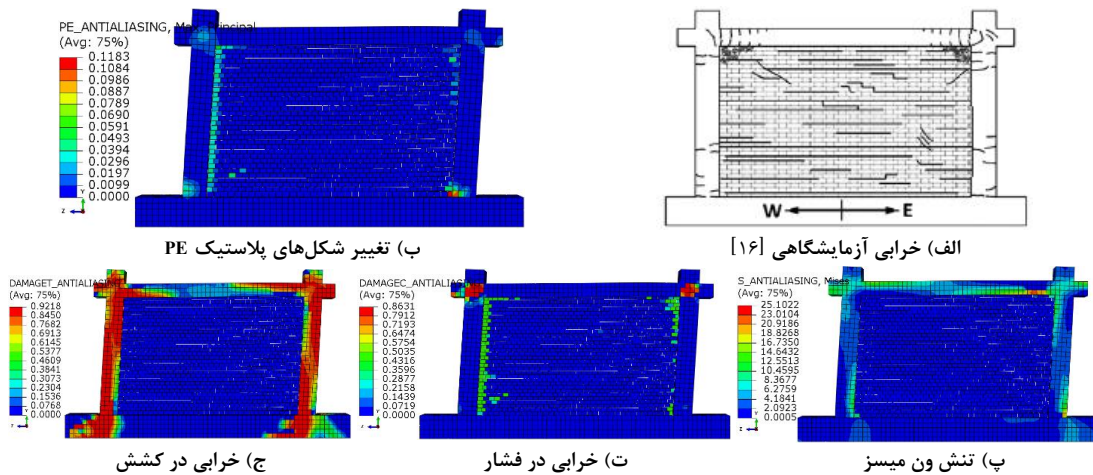
Fig. 17. Experimental and finite element of damage pattern of reference specimen NS-T100-P0.1-SOLID-V with relative displacement 4.3%. a) Experimental damage, b) Plastic deformation, c) Mises stress, d) Compression damage, e) Tension damage
