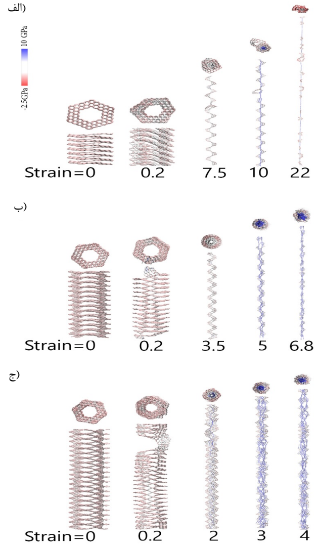
Fig. 4. (the comparison of tensile behavior between sample 1 with 1) one-layer b) 2 layers c) 3 layers. The color of atoms related to their stress in tensile direction.)
