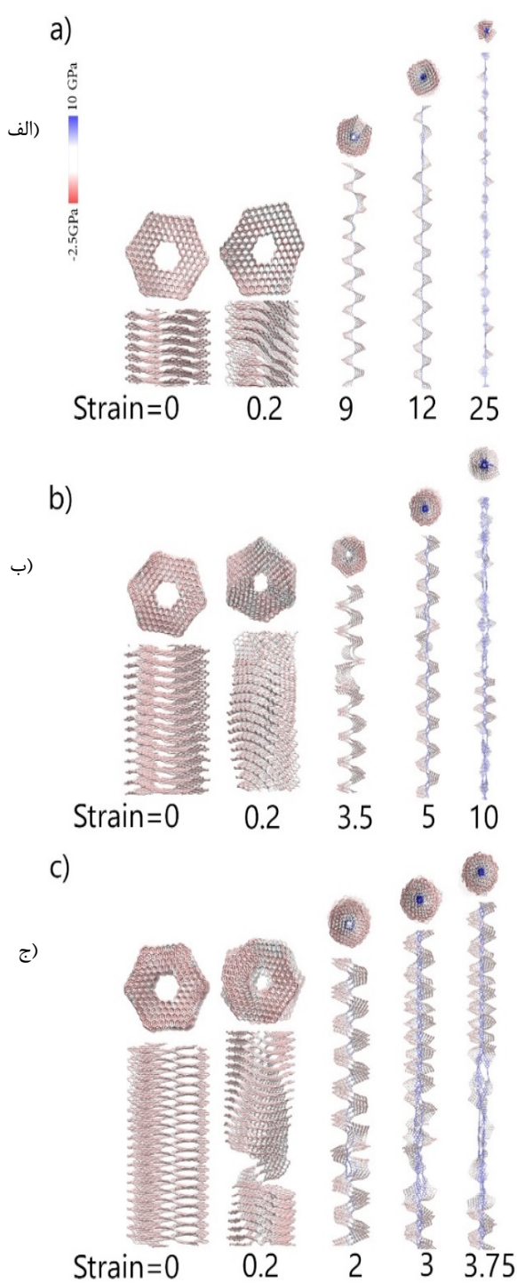
Fig. 5. (the comparison of tensile behavior between sample 2 with 1) one-layer b) 2 layers c) 3 layers. The color of atoms related to their stress in tensile direction.)
