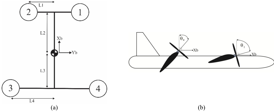
Fig. 6. The quad single TR configuration for the dynamic modeling from (a) the top view, (b) the side view.
