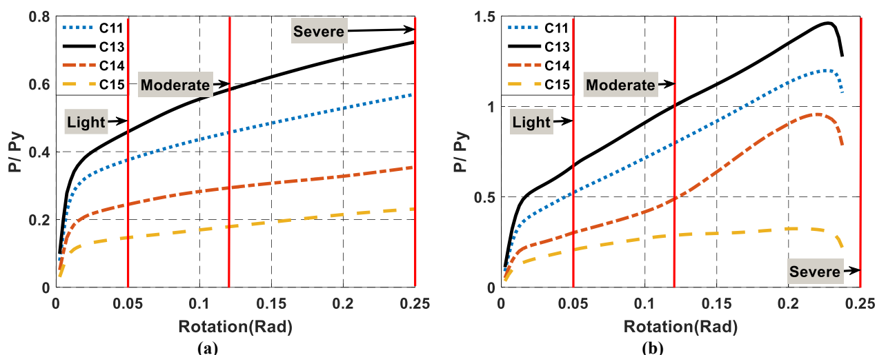
Fig. 8. The ratio of P/P_y in the columns adjacent to the removed interior column C12 under three damage states: (a) Without catenary action; (b) With catenary action.
