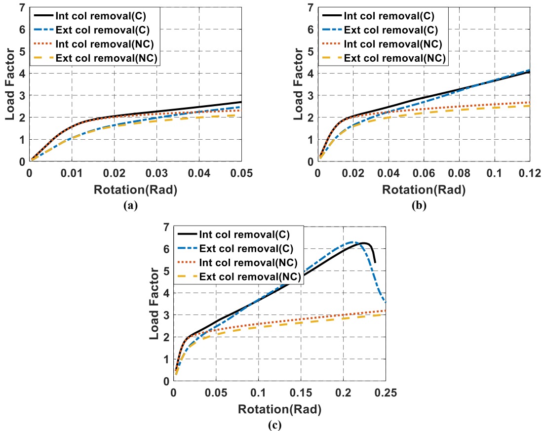
Fig. 6. Load factor for the structural model in the removal of exterior and interior columns with catenary action (C) and without catenary action (NC) in different damage states: (a) Light; (b) Moderate; (c) Severe.
