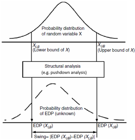
Fig. 5. The process of performing the tornado analysis [31].
