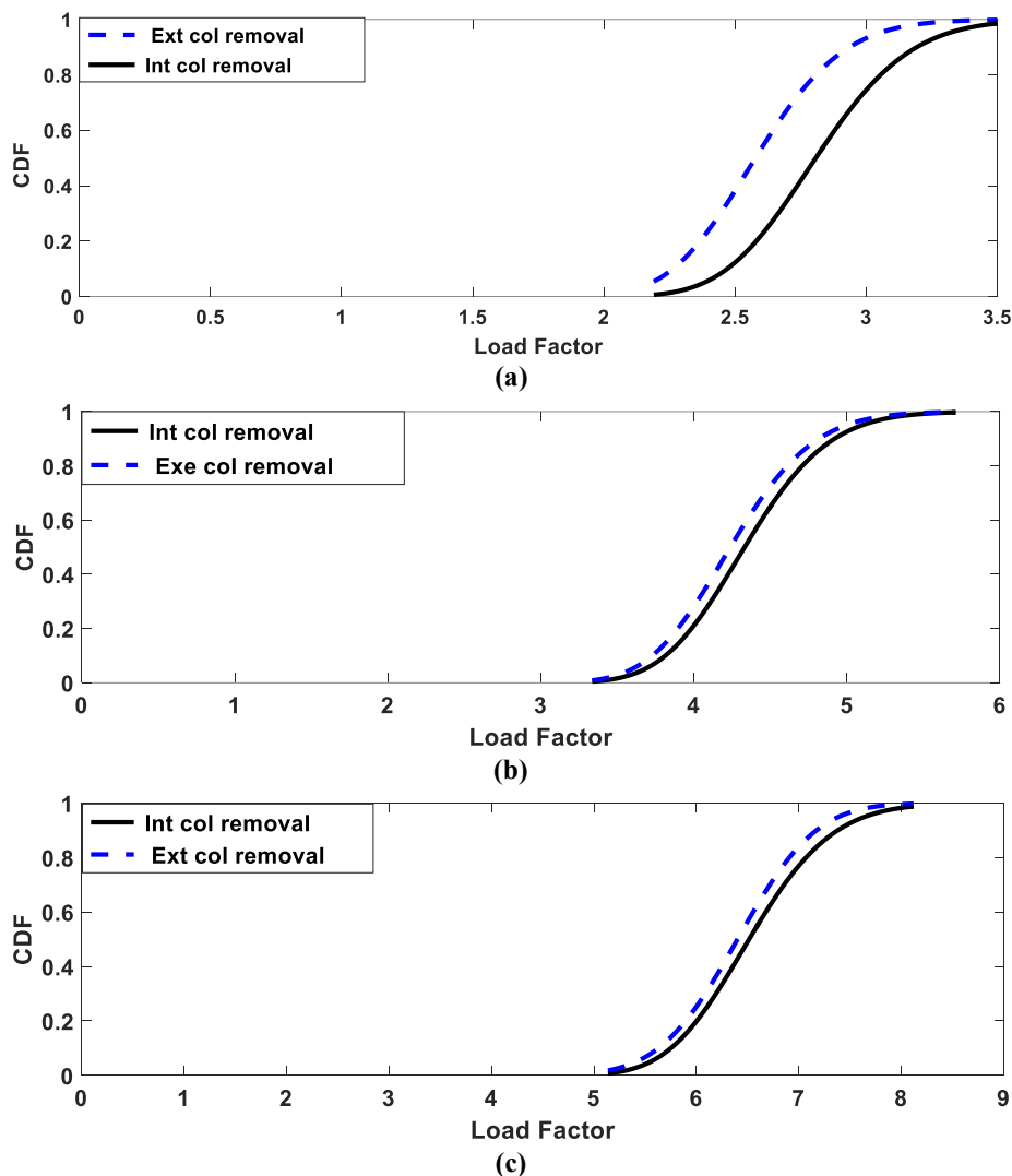
Fig. 11. Cumulative distribution function (CDF) curves of the load factor in limit states: (a) Light; (b) Moderate; (c) Severe.
