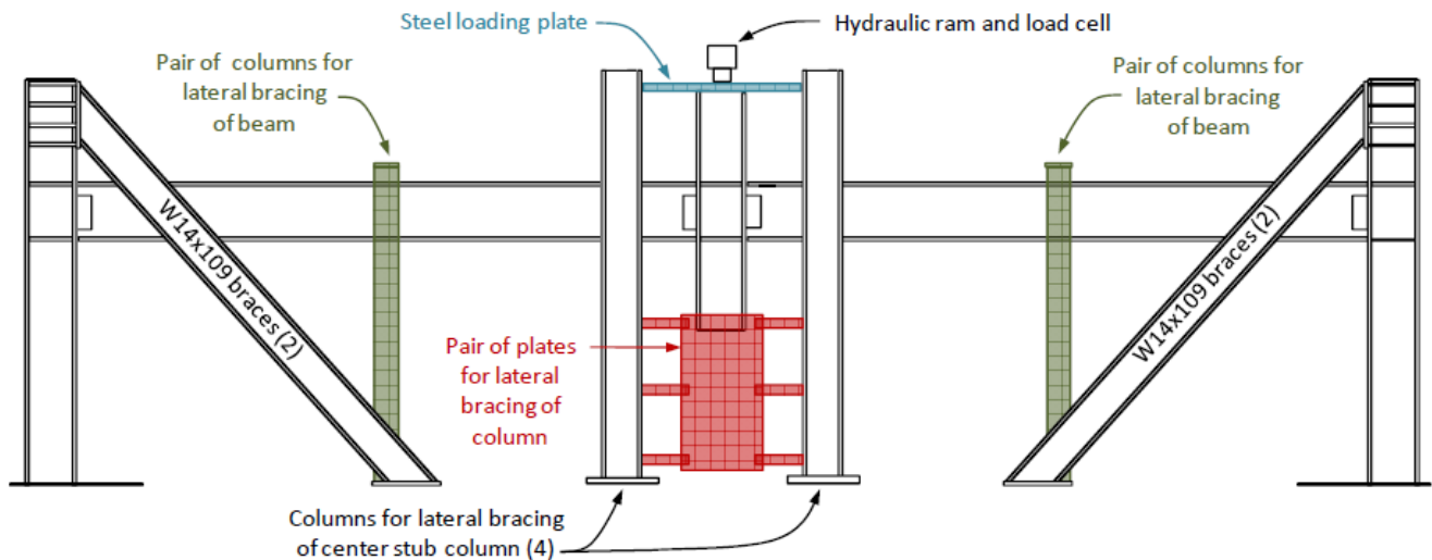
Fig. 1. Details of test setup for specimen [20].
