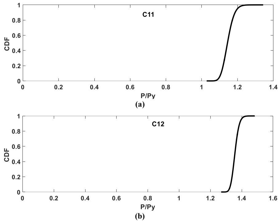
Fig. 12. Cumulative distribution function (CDF) curves of the ratio P/P_y in the adjacent column to the damaged column in both the exterior and interior column removal scenarios in the severe limit state: (a) column C11; (b) column C12
