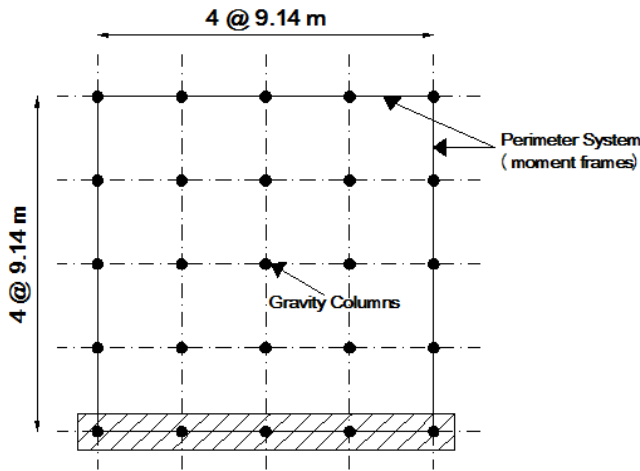
Fig. 3. Plan view of the 8-story model [21].
