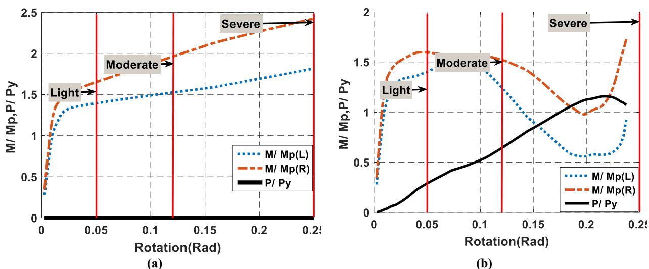
Fig. 9. The ratio M/M_p or P/P_y in beam 101 above the interior removed column C12 under three damage states: (a) Without catenary action; (b) With catenary action.
