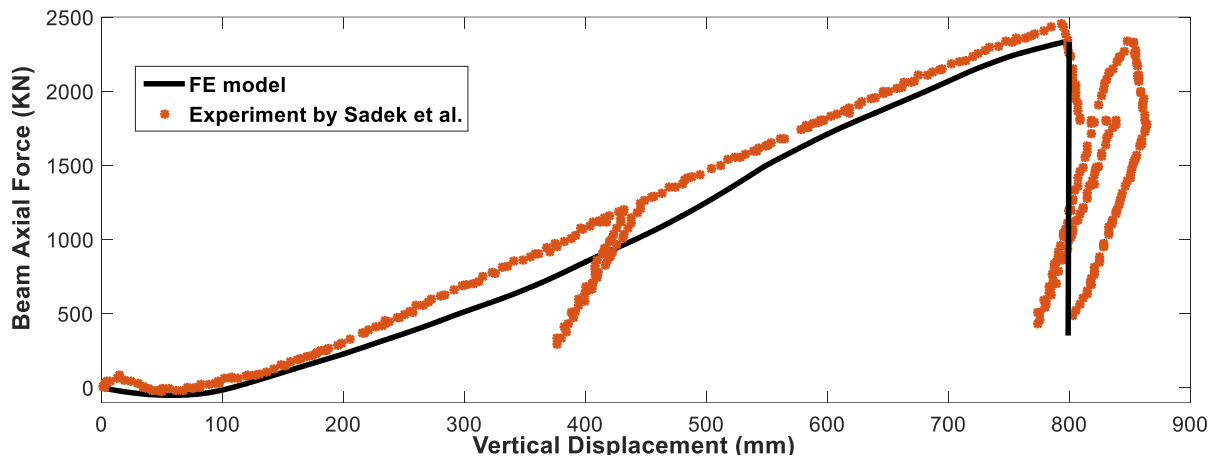
Fig. 2. Comparison of the results of the numerical model and laboratory test for the axial force created in the beams.
