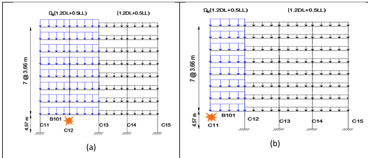
Fig. 4. Load combination in pushdown analysis: (a) interior column removal; (b) exterior column removal.
