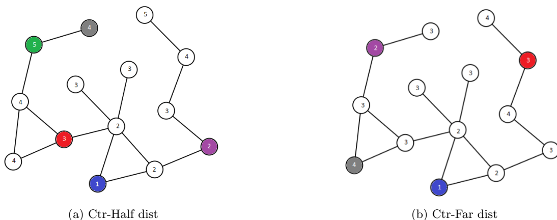
Figure 1: Comparison of Ctr-Half dist and Ctr-Far dist. Activators are colored vertices and the number inside each vertex shows the time step it burns.
