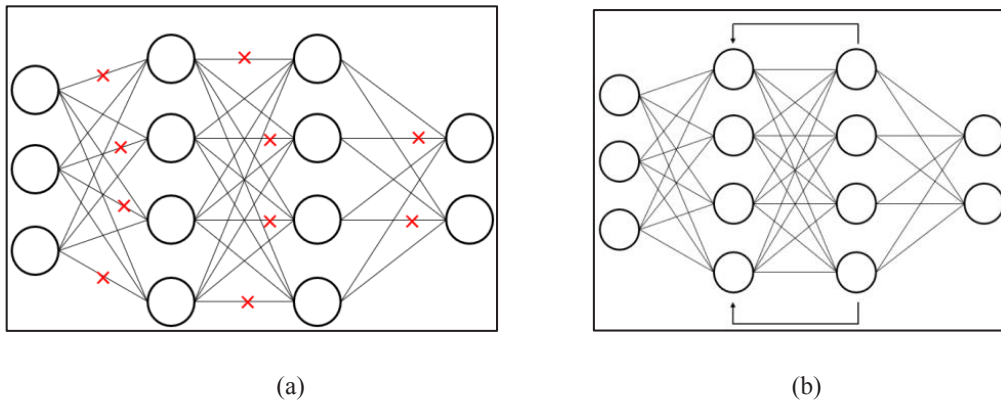
Fig. 3. (a) convolutional neural networks schematic (b) recurrent neural networks schematic
