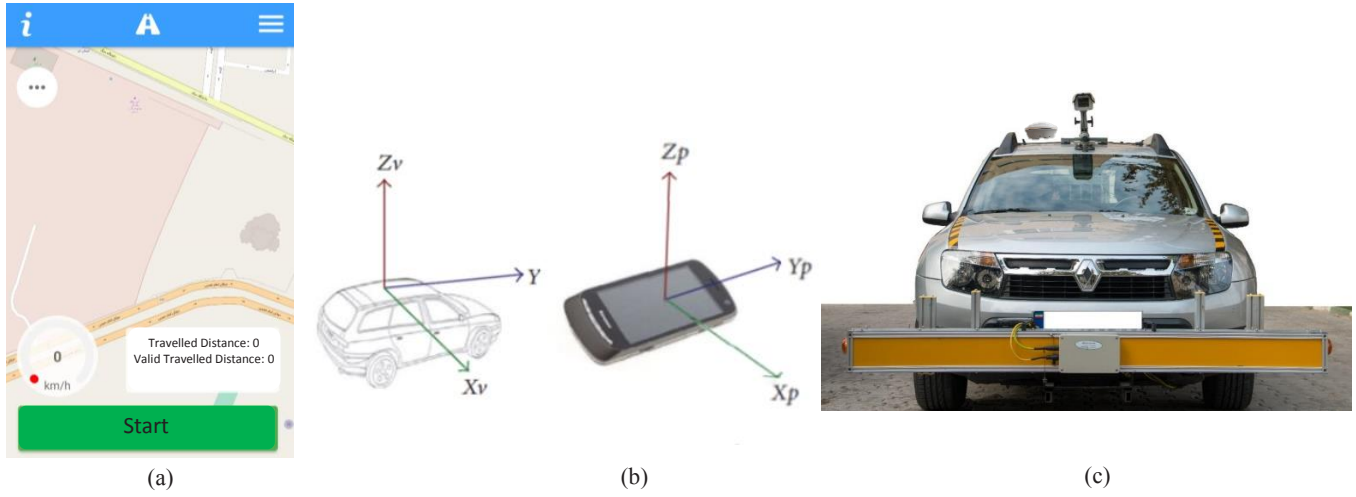
Fig. 2. (a) the application developed to collect and send data to the server (b) smartphone and vehicle coordinate systems (c) RSP (the Road Surface Profiler)
