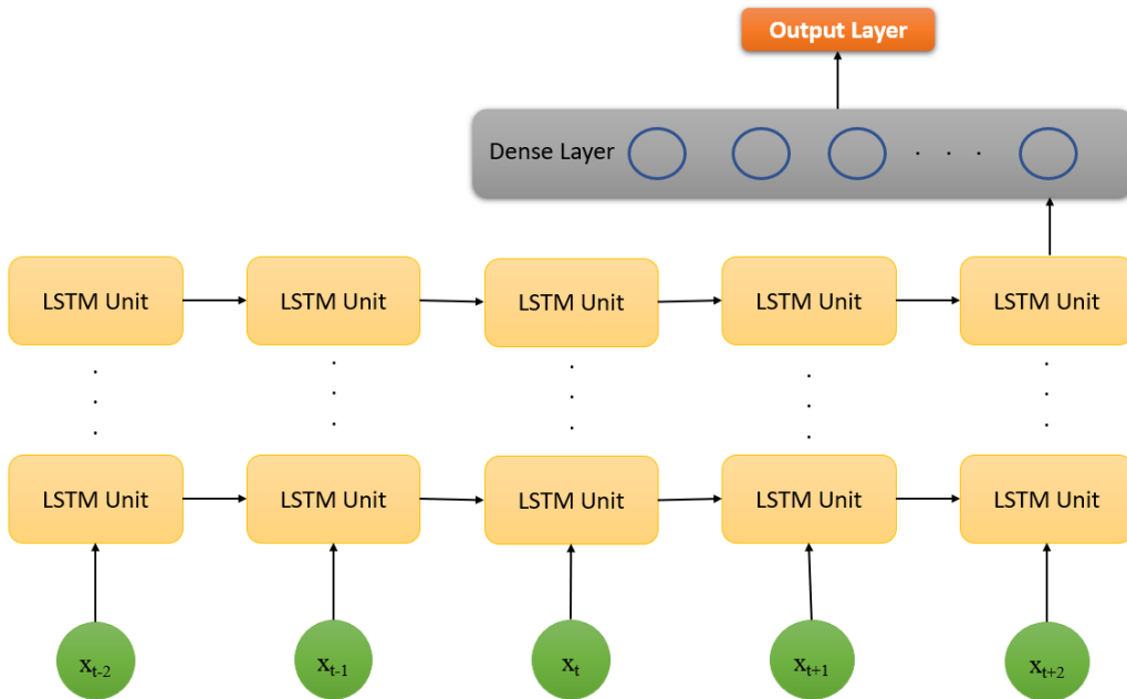
Fig. 7. A recurrent neural networks
