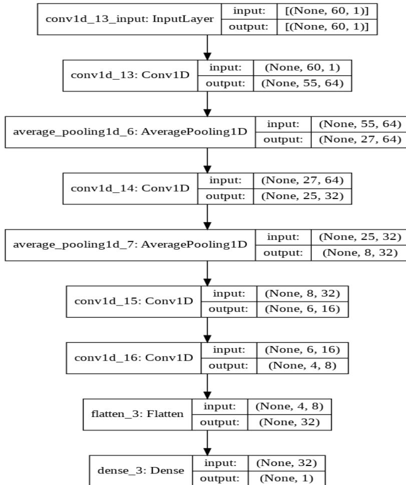
Fig. 4. A sample of a convolutional neural network used to estimate longitudinal and angular accelerations
