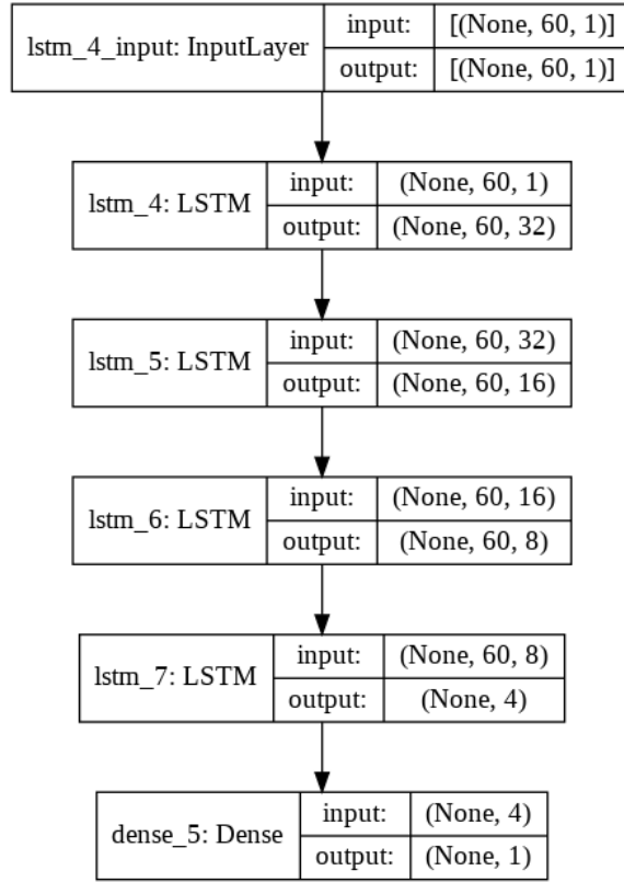
Fig. 6. A sample of a recurrent neural network used to estimate longitudinal and angular accelerations
