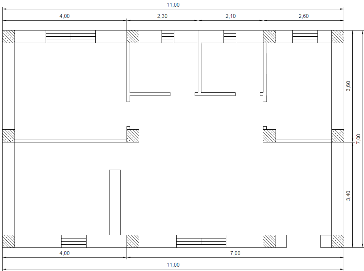
Fig. 1. Plan of the investigated building.
