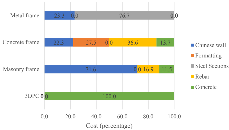
Fig. 4. The cost of different manufacturing methods by item (percentage)
