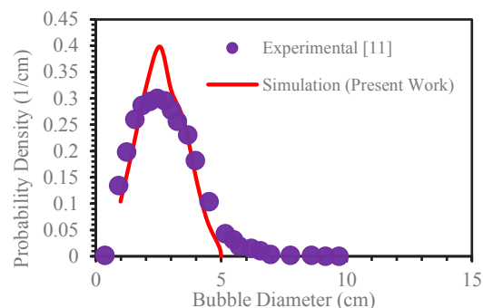
Fig. 2. Comparison of the size distribution of bubbles at a height of 90 mm from the bottom of the bed and a velocity of 3.4 times the minimum fluidization velocity between simulation and experimental data [11]
