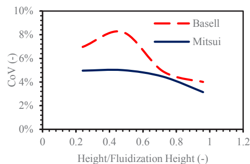
Fig. 3. Comparison of the CoV related to the time-averaged volume fraction of the gas phase
