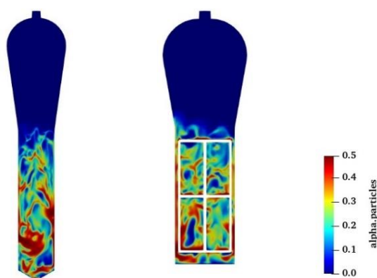
Fig. 1. Contour of volume fraction of particles obtained from the simulation of the industrial reactor at t=30 s
