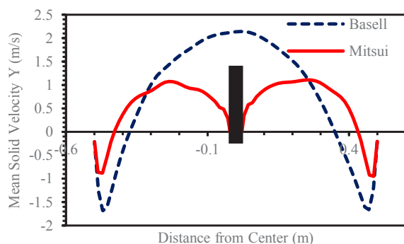
Fig. 4. Comparison of the time-averaged solid phase velocity (from 10 to 30 seconds) in the axial direction and at a normal height of 0.72.
