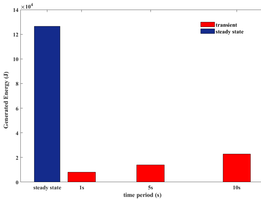
Fig. 1. Generated energy in wire heater at durations of 1, 5, and 10s and steady mode
