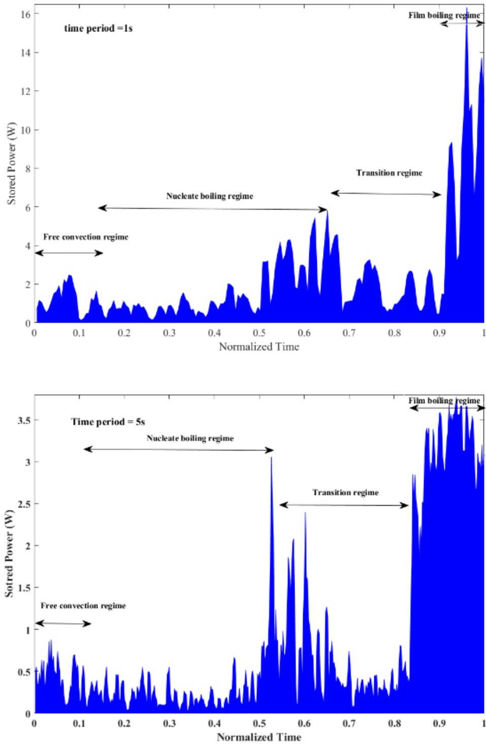
Fig. 5. stored energy rate at 1, 5, and 10s (Continued).
