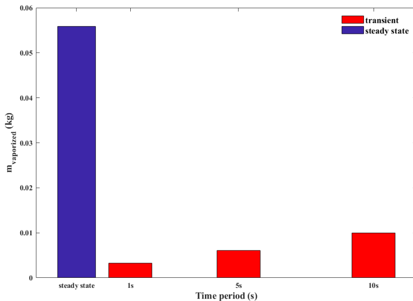
Fig. 8. vaporized water amount during experiments in transient and steady modes.
