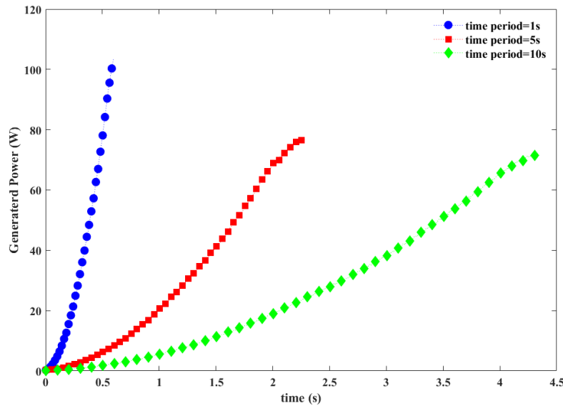
Fig. 3. generated energy rate versus non-normalized time for durations of 1, 5, and 10s
