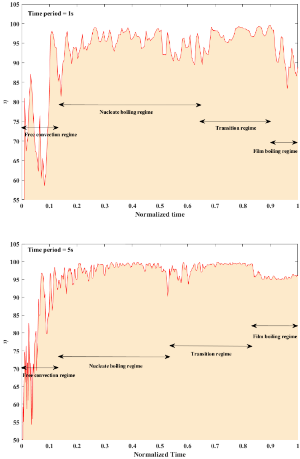
Fig. 12. Coolant performance versus normalized time for duration of 1s, 5s, and 10s(Continued).
