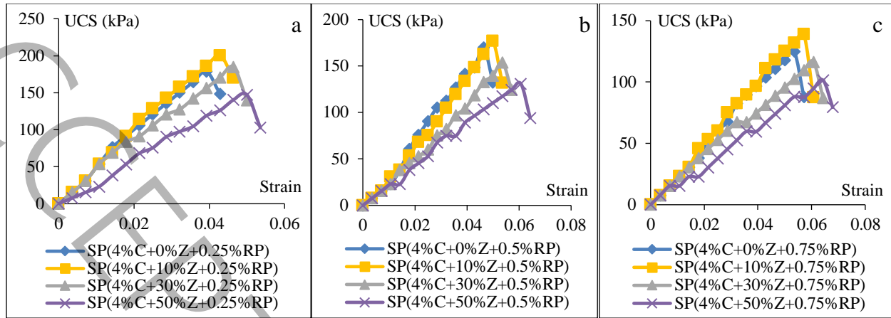
Fig. 11. Stress-strain diagram of stabilized samples (SP) by cement, zeolite and rubber powder replacement in curing period of 28 days – a: 0.25% rubber powder, b: 0.5% rubber powder, c: 0.75% rubber powder
