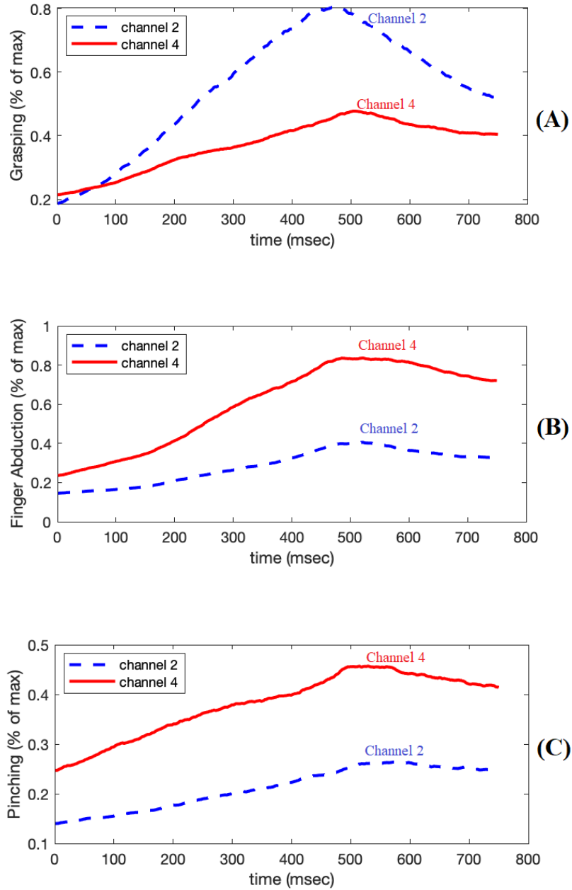
Fig. 5. The average signal of all subjects in two channels #2 and #4 for three movements: A) grasping B) abduction of fingers C) pinching; The blue curve represents channel #2, and the red curve is channel #4
