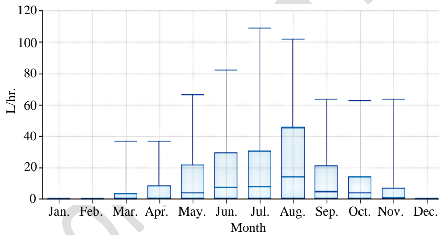
Fig. 7. Fuel consumption amount in C_B
