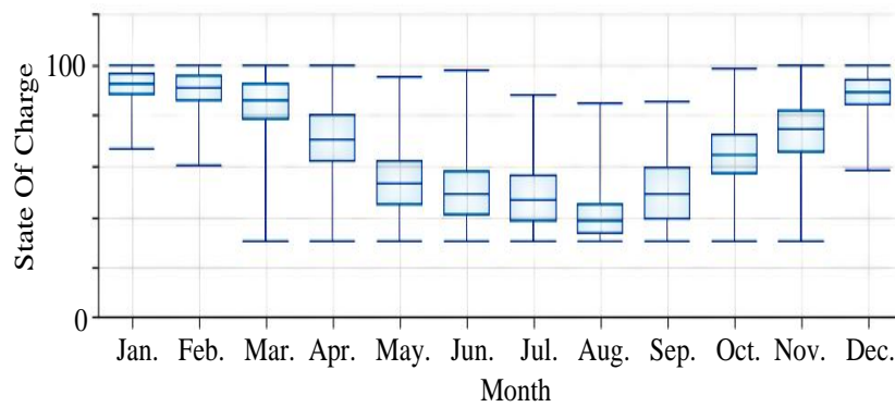
Fig. 9. State of charge in C_B
