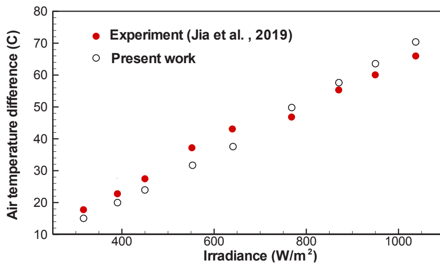
Fig. 7. Validation of the numerical results with experiment, \dot{m} = 0.0146 \text{ kg/s}
