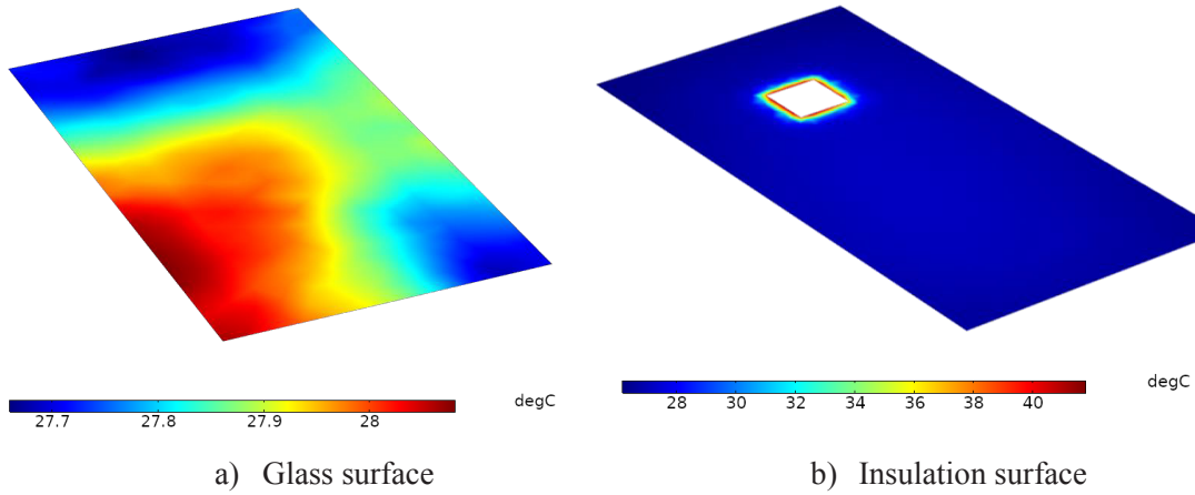
Fig. 13. Temperature distributions over the outer surfaces of the glass cover and insulation
