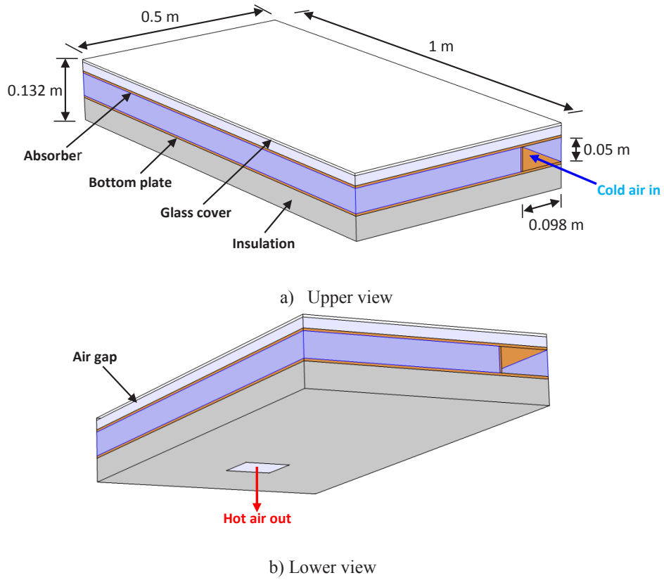
Fig. 1. Schematic of the SAH
