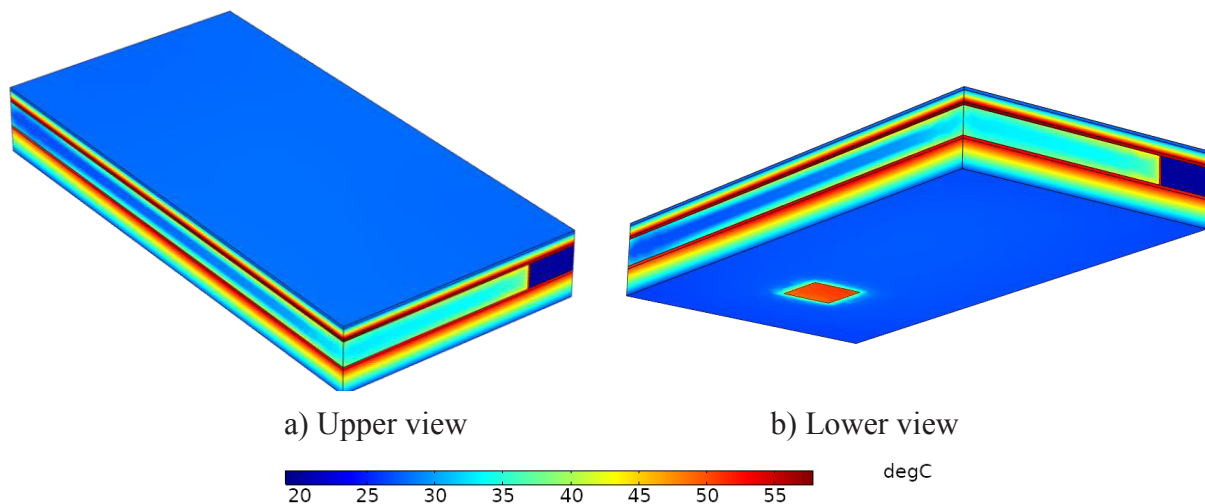
Fig. 9. Isotherm plots inside the SAH
