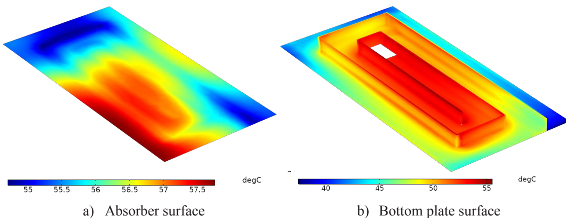
Fig. 11. Temperature distribution over the absorber and bottom plate surfaces
