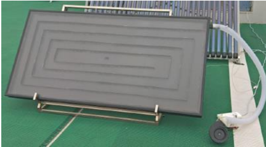
Fig. 6. Photo of the test system [16]
