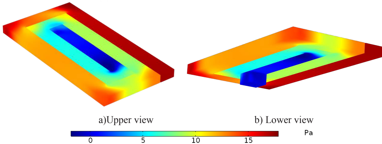
Fig. 15. Isobar contours for forced convection airflow
