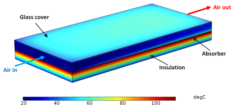
a) Isotherm plots inside the conventional plane SAH
