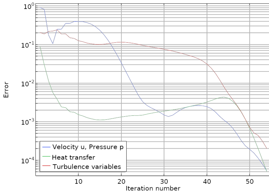
Fig. 4. Variations of the residuals during iterative steps
