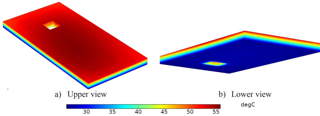
Fig. 12. Isotherm plots inside the insulation layer
