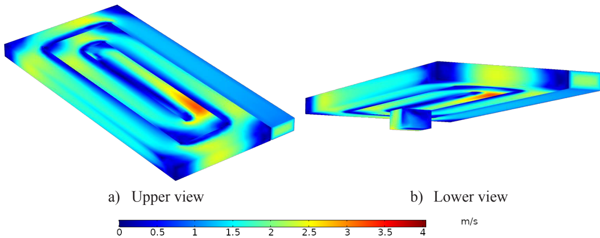
Fig. 8. Velocity magnitude contour plot
