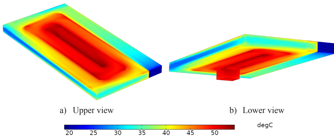
Fig. 10. Isotherm plot inside the convection airflow
