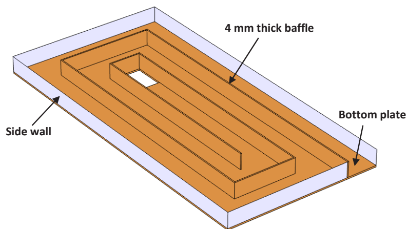
Fig. 2. Bottom plate including the air passageway
