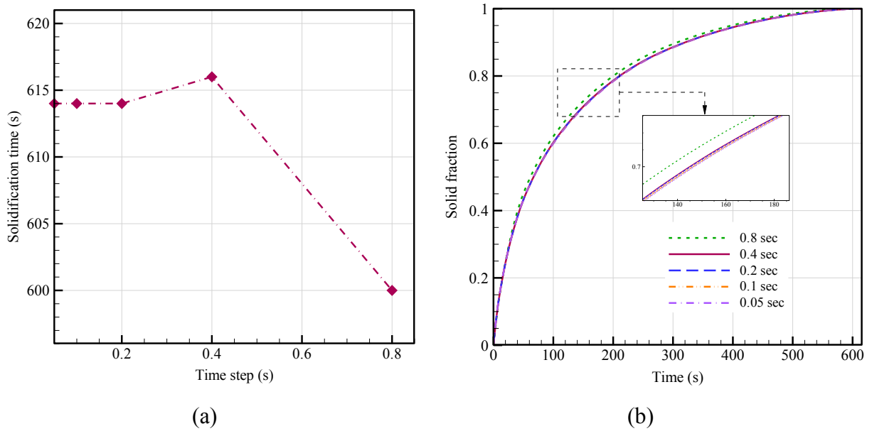
Fig. 4. Time step independence study.
