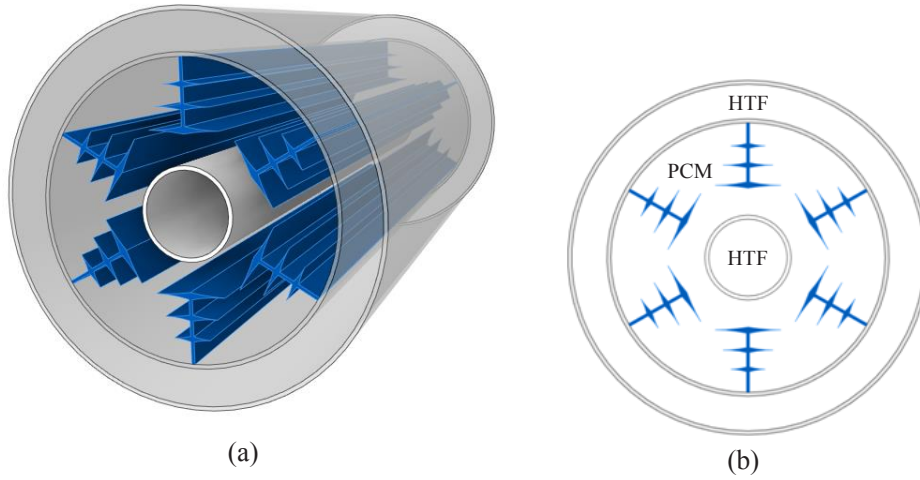
Fig. 1. The triplex tube LHTES unit: (a) 3D schematic view, (b) 2D cross section.
