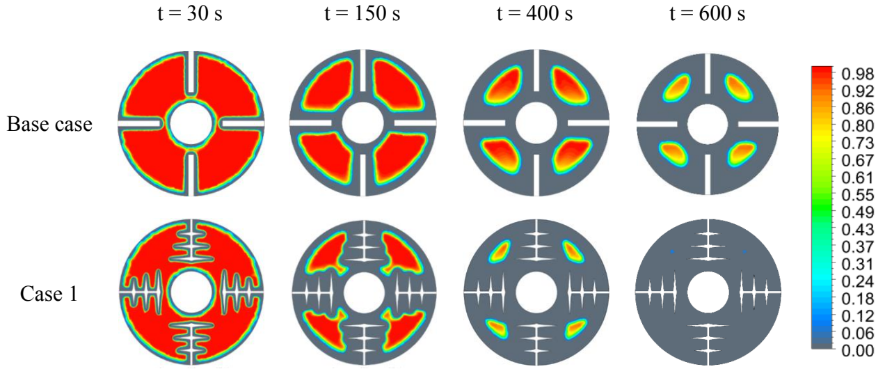
Fig. 6. Contour plot of liquid fraction for the straight fins and longitudinal-parabolic fins.
