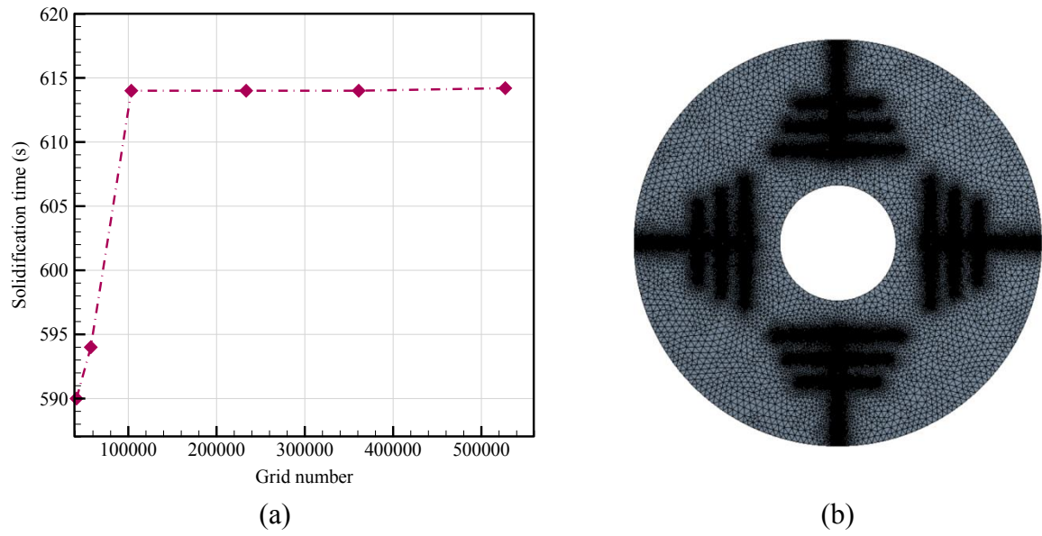
Fig. 3. (a) Grid size independence verification, (b) the computational grid.
