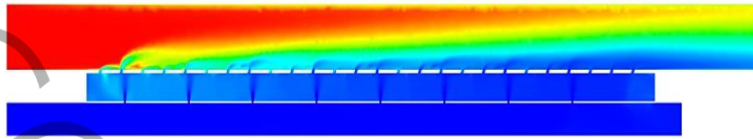
Fig. 15. Cooling efficiency distribution contour for the optimal geometry with a blowing ratio of 1
