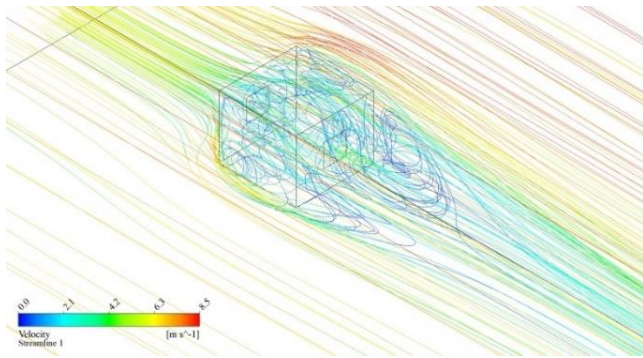
Fig. 3. 3D contour of flow lines inside and outside the building model
