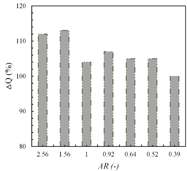
Fig. 2. The percentage increase in volumetric flow rate for models with varying window dimensions at a 0° wind angle compared to the reference model
