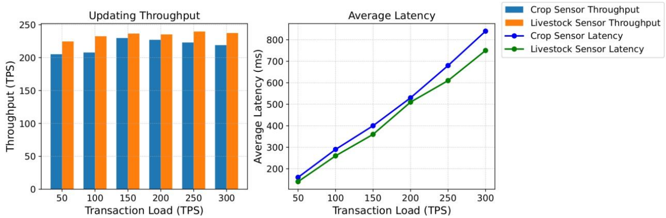
Fig. 5. Throughput and Average Latency for updating sensor data.
