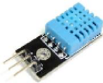
Fig. 7. The DHT11 Temperature Area Sensor.
