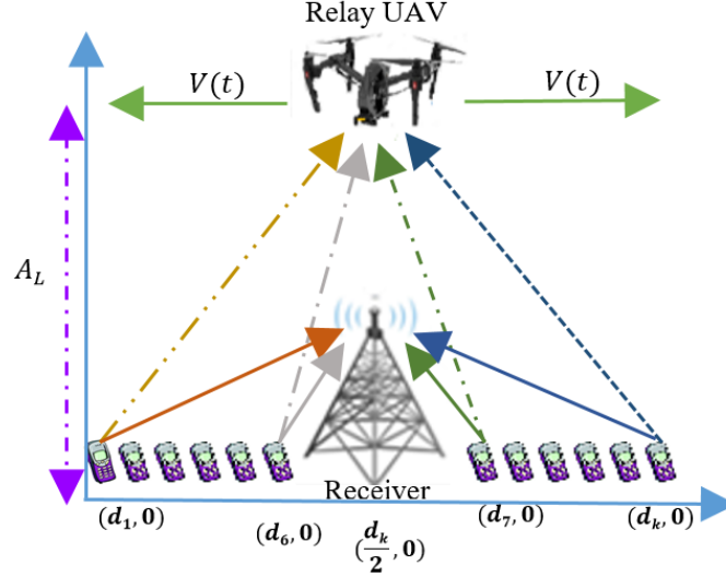
Fig. 1. A System With K Terrestrial Transmitters, Terrestrial Receiver, and UAV Relay.
