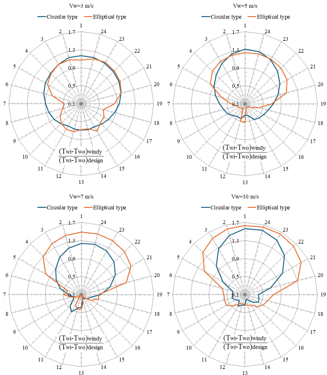
Fig. 1. Dimensionless distribution of outlet water temperature leaving radiator at different wind velocities.
